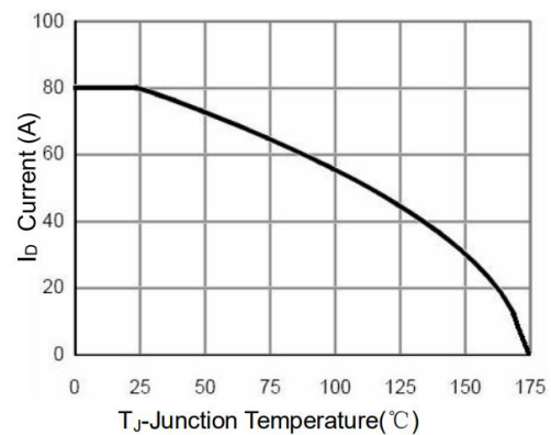
Figure 10: Maximum Continuous Drian Current vs. Case Temperature
