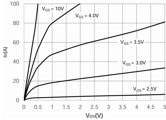
Figure 1: Output Characteristics
