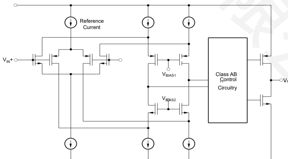
Figure 2. Simplified Schematic.
