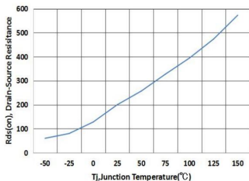
图 3 导通电阻与温度曲线 Fig3 Normalized Resistance Vs. Temperature
