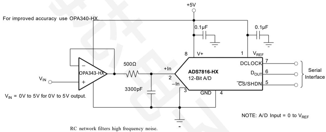
Figure 5. OPA343NA-HX in Noninverting Configuration Driving ADS7816-HX.
