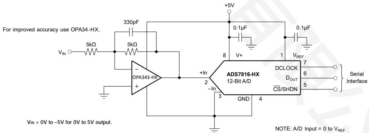
Figure 6. OPA343NA-HX in Inverting Configuration Driving ADS7816-HX.
