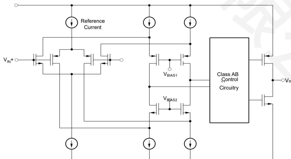
Figure 2. Simplified Schematic.
