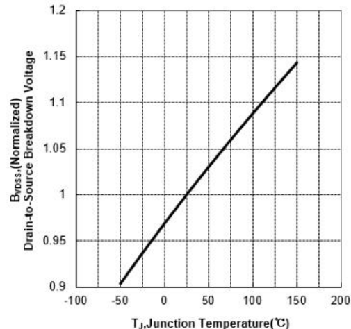
Figure 9 Typical Breakdown Voltage vs Junction Temperature
