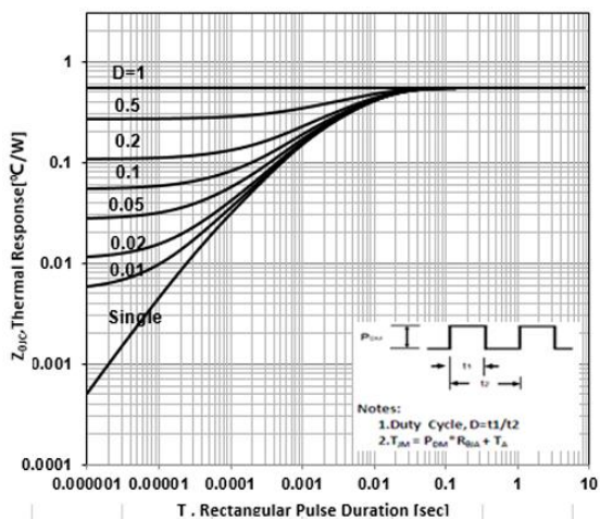
Figure 3a Max Thermal Impedance (No FullPAK)
