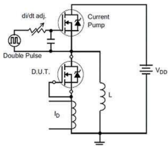
Figure 16 Diode Reverse Recovery Test Circuit
