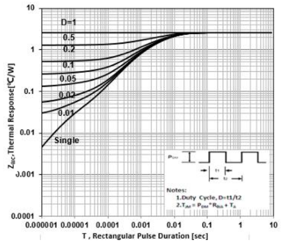
Figure 3b Max Thermal Impedance (FullPAK)
