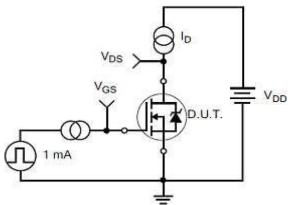
Figure 12 Gate Charge Test Circuit
