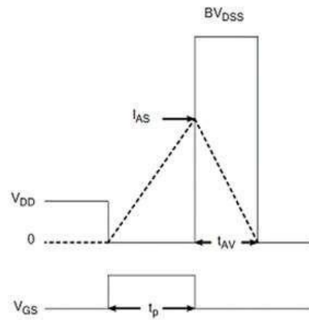
Figure 19 Unclamped Inductive Switching
