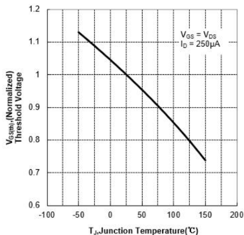
Figure 8 Typical Threshold Voltage vs Junction Temperature
