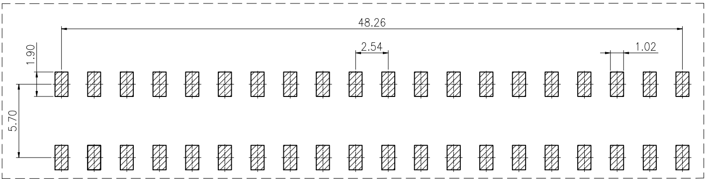
PCB LAYOUT
