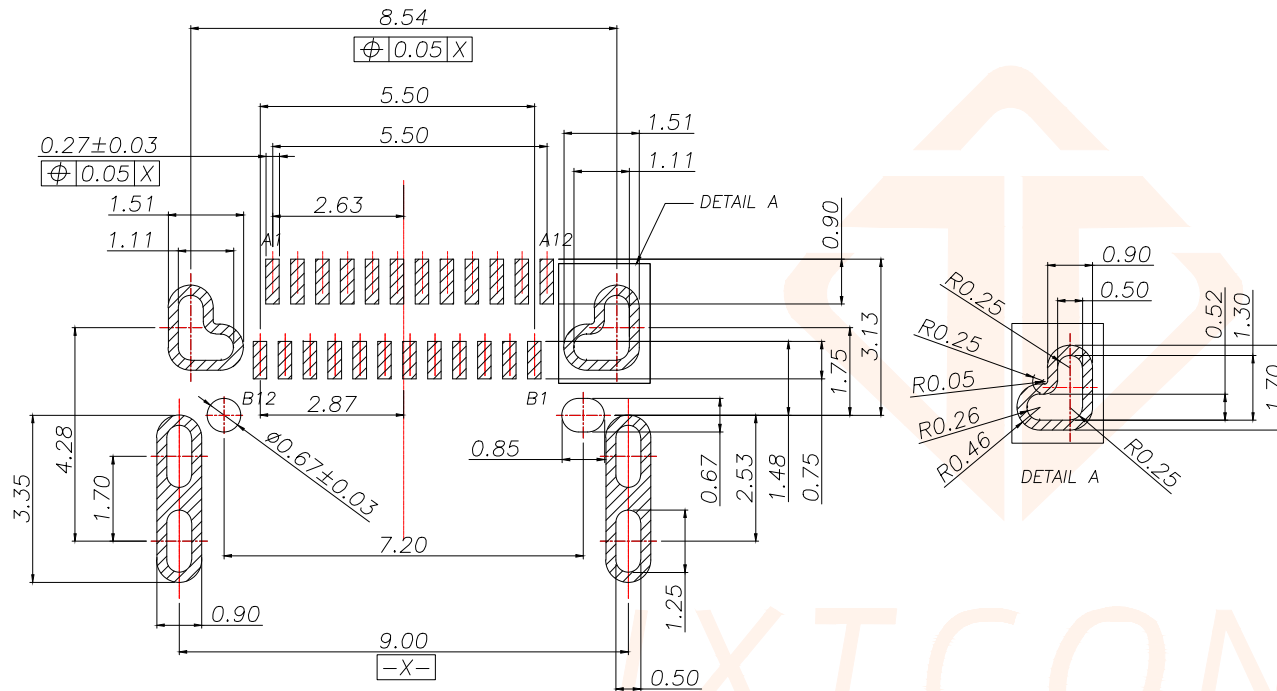
SCALE 2:1 RECOMMENDED PCB LAYOUT(TOP VIEW) Thickness 1.0mm (TOLERANCE=±0.05mm)
