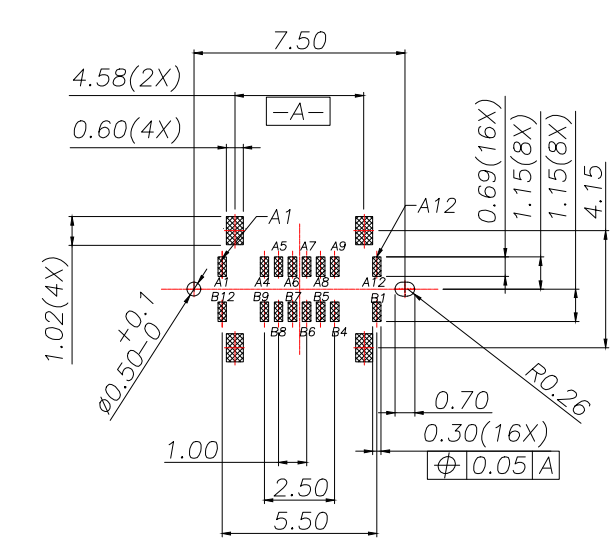
RECOMMENDED PCB LAYOUT(TOP VIEW) THICKNESS 0.8±0.10MM;DEFAULT TOLERANCE:±0.05
