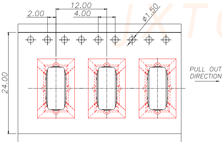
DETAIL X
