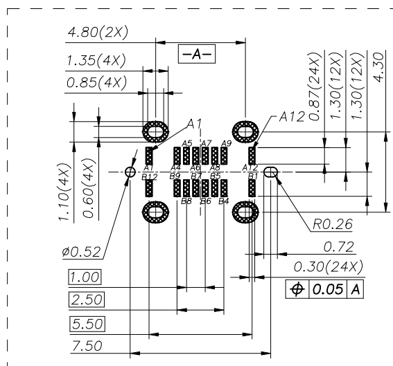
RECOMMENDED PCB LAYOUT(TOP VIEW) THICKNESS 1.0±0.10MM;DEFAULT TOLERANCE:±0.05
