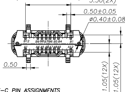
USB TYPE-C PIN ASSIGNMENTS
