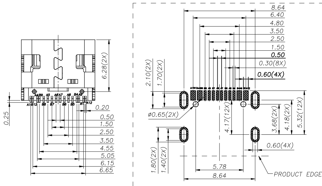
RECOMMENDED PCB LAYOUT(TOP VIEW)
