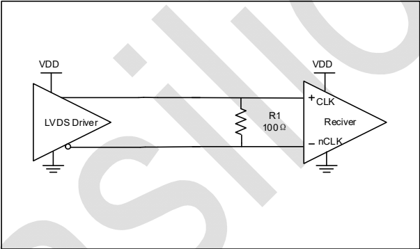
Figure3.LVDS Driver
