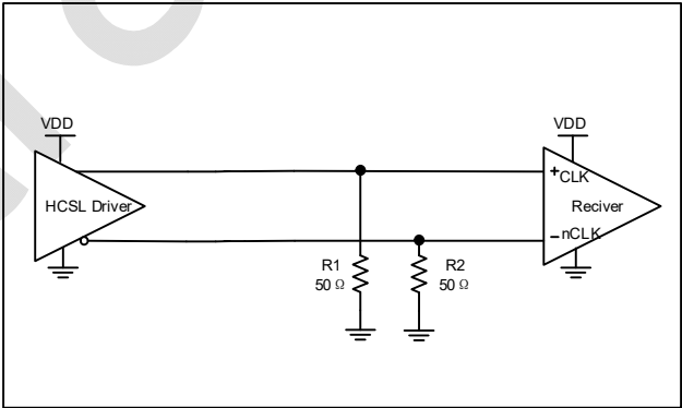
Figure4.HCSL Driver
