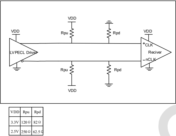
Figure2.LVPECL Driver
