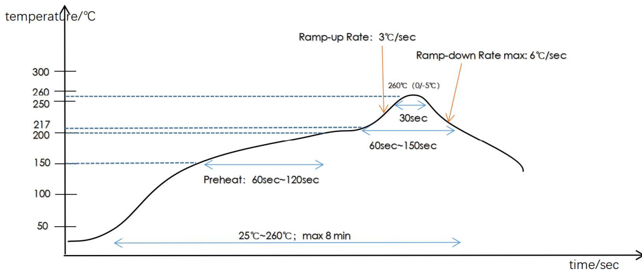
Figure5: Recommended Temperature(PB-Free)
