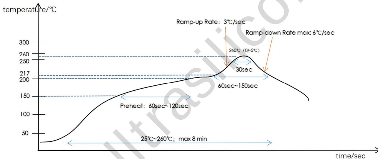
Figure11: Recommended Temperature(PB-Free)
