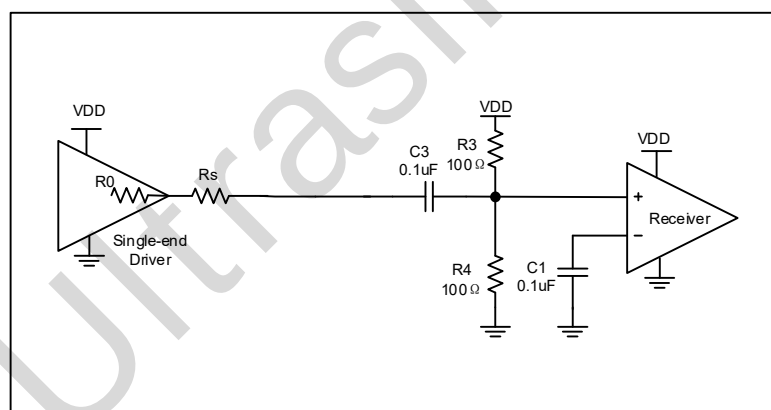
Figure4.Single-ended input
