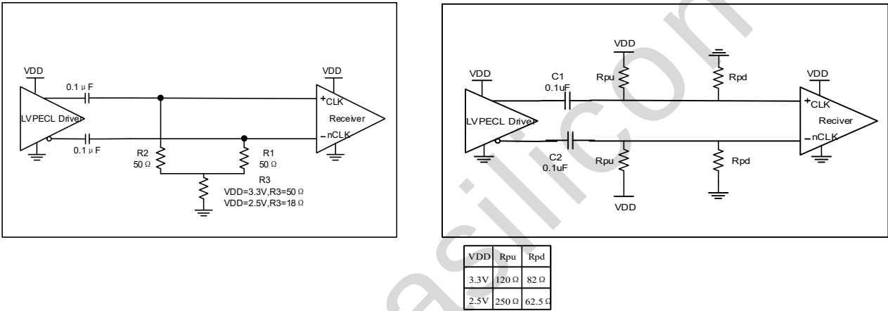
Figure5.LVPECL Driver(AC)
