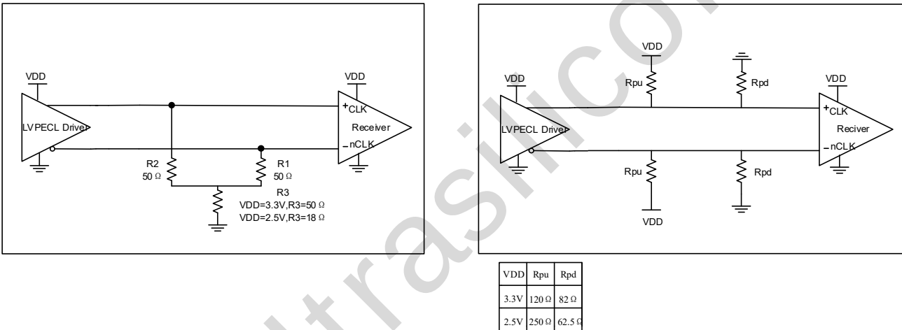
Figure6.LVPECL Driver(DC)
