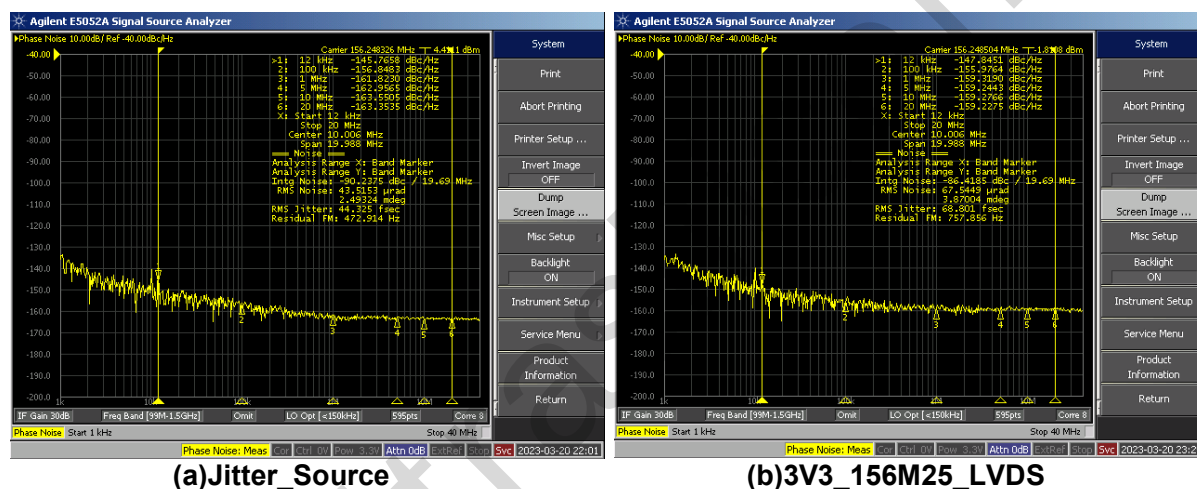
Figure 1 .RMS_Jitter_3V3= \sqrt{68^2-44^2} =51fs
