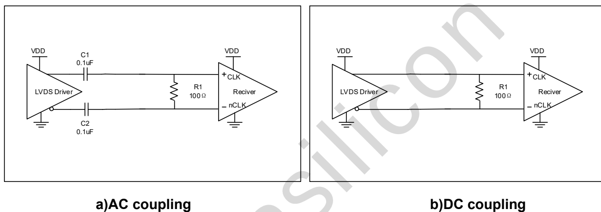
Figure7.LVDS Driver
