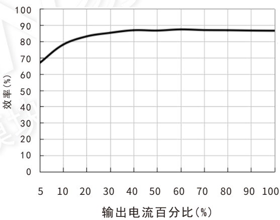
效率Vs输出负载(V in =48V)
