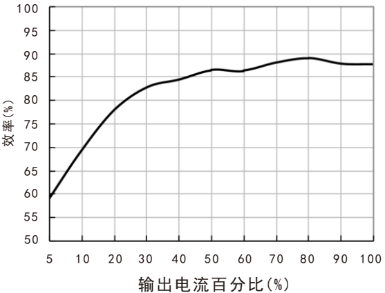
效率Vs输出负载(V in =48V)
