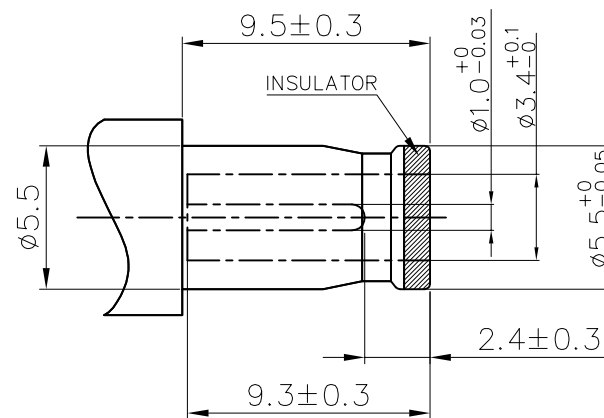
MATE PLUG
