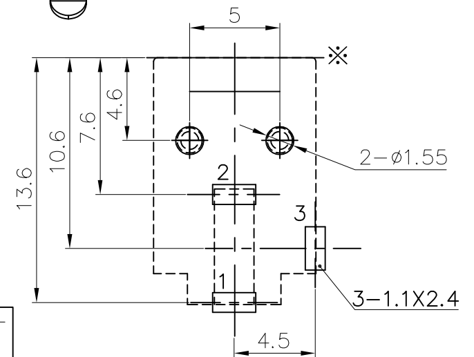
PCB Holes diagram Bottom View
