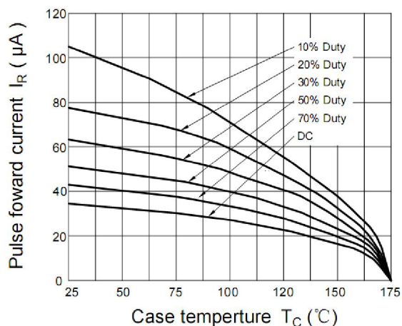
Figure 3. Load current
