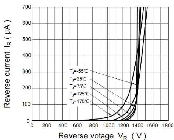
Figure 2. Reverse Characteristics
