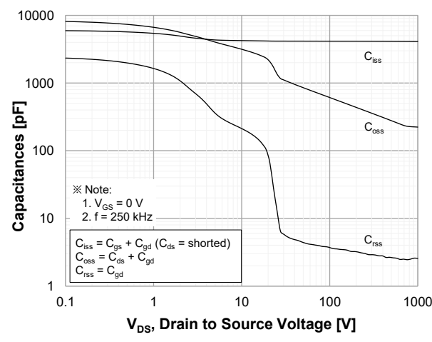
Figure 12. Capacitance Characteristics
