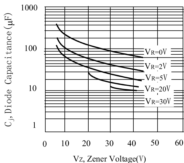
Fig.3 Junction Capacitance vs V_z , Zener Voltage
