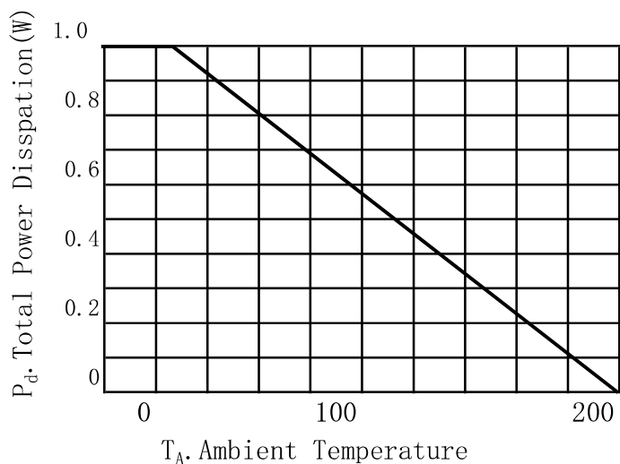
Fig.1 Power Dissipation vs Ambient Temperature
