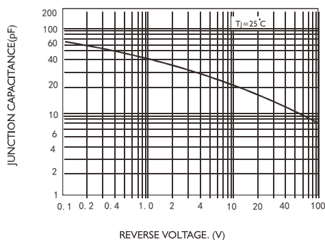
FIG.5-TYPICAL JUNCTION CAPACITANCE
