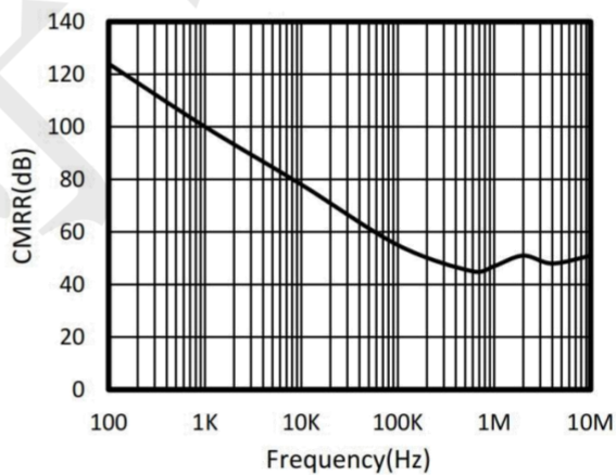
Figure 4. Common-Mode Rejection Ratio vs Frequency
