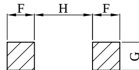
( PCB Pattern )
