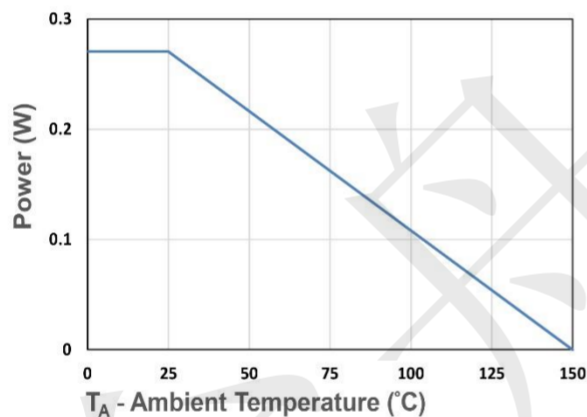
Figure 9. Power Dissipation
