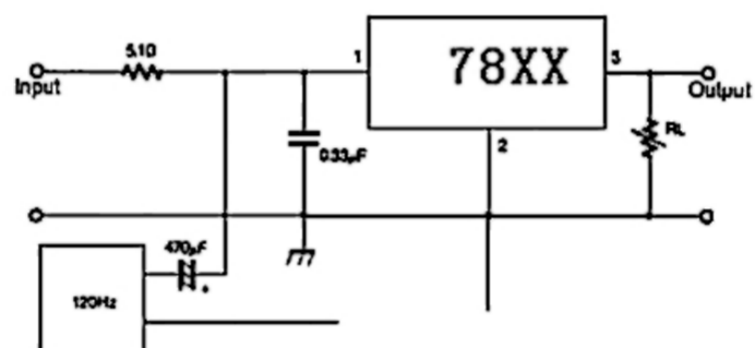
Ripple Rejection
