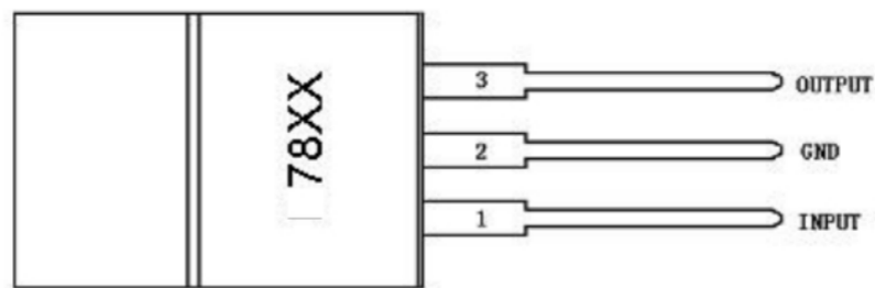
78XX(TO220-3)
