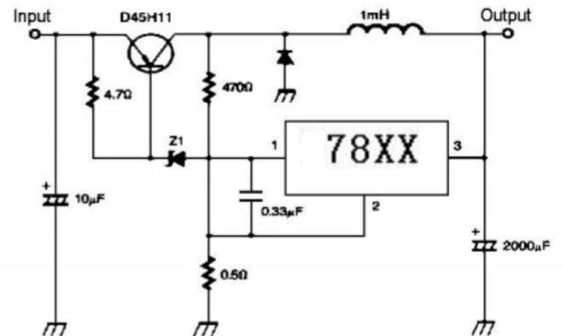
Switching Regulator
