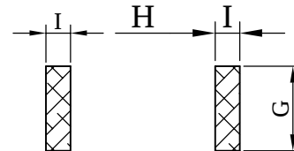
( PCB Pattern )
