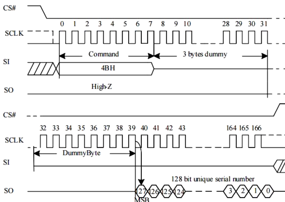
Figure 10-58 Read Unique ID (RUID) Sequence (Command 4BH)
