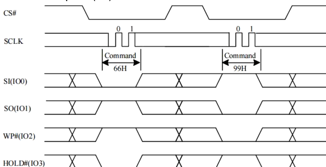
Figure 10-56b Reset Sequence (QPI)
