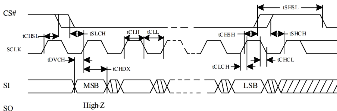
Figure 5-4a Serial Input Timing in non-DTR Mode
