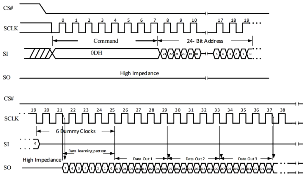
Figure 10-23f DTR 2IO Read with DLP bits output Sequence
