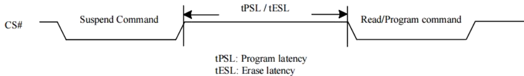
Figure 10-48a Suspend to Read/Program Latency (QPI)
