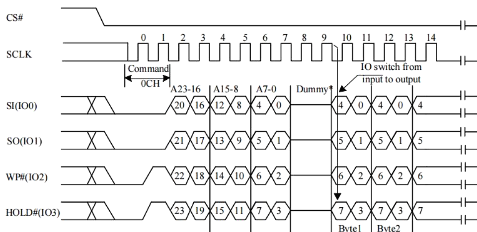
Figure 10-21 Burst Read with Wrap Sequence (QPI)
