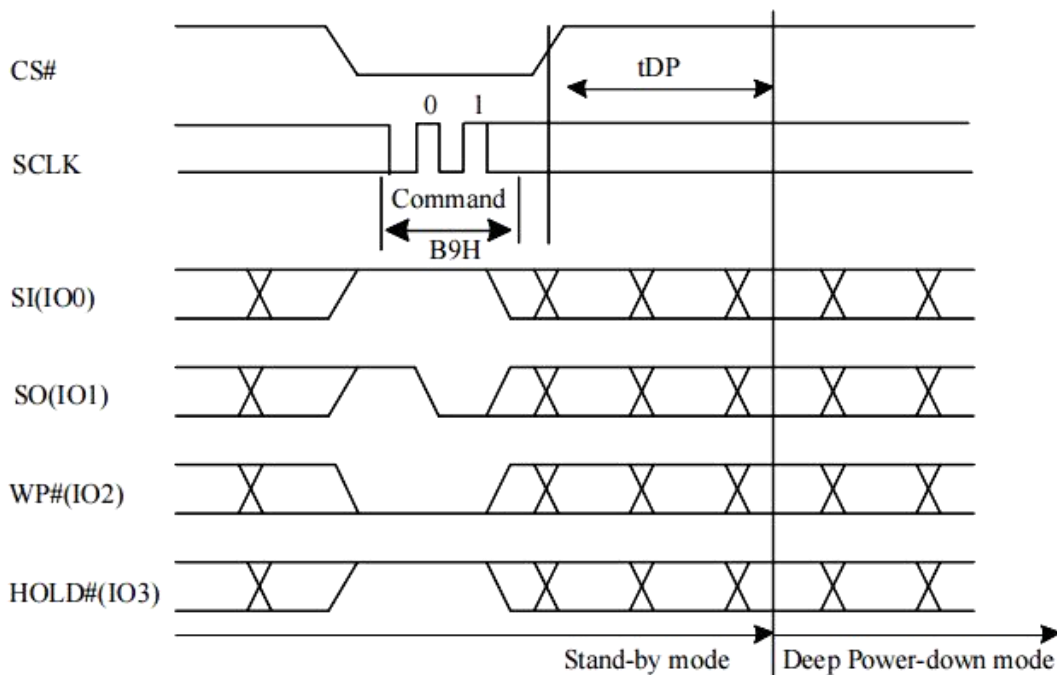
Figure 10-41a Deep Power-down (DP) Sequence (QPI)
