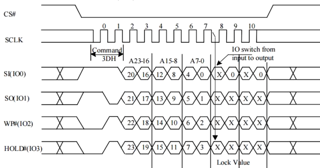
Figure 10-53a Read Block Lock Status (QPI)
