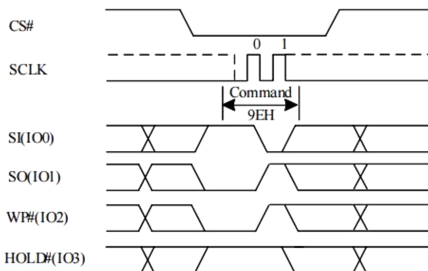
Figure 10-33a Buffer Clear Sequence (QPI)
