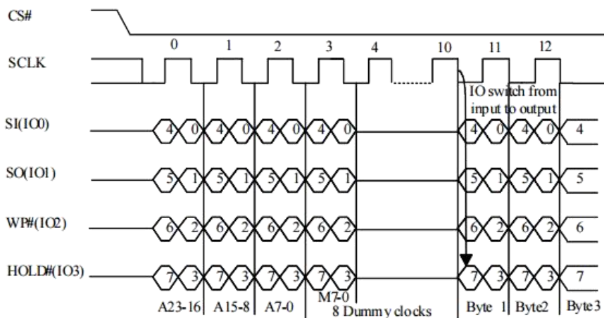
Figure 10-18a DTR 4IO Continuous Read Mode Sequence (Command ED M5-4 = (1,0))
