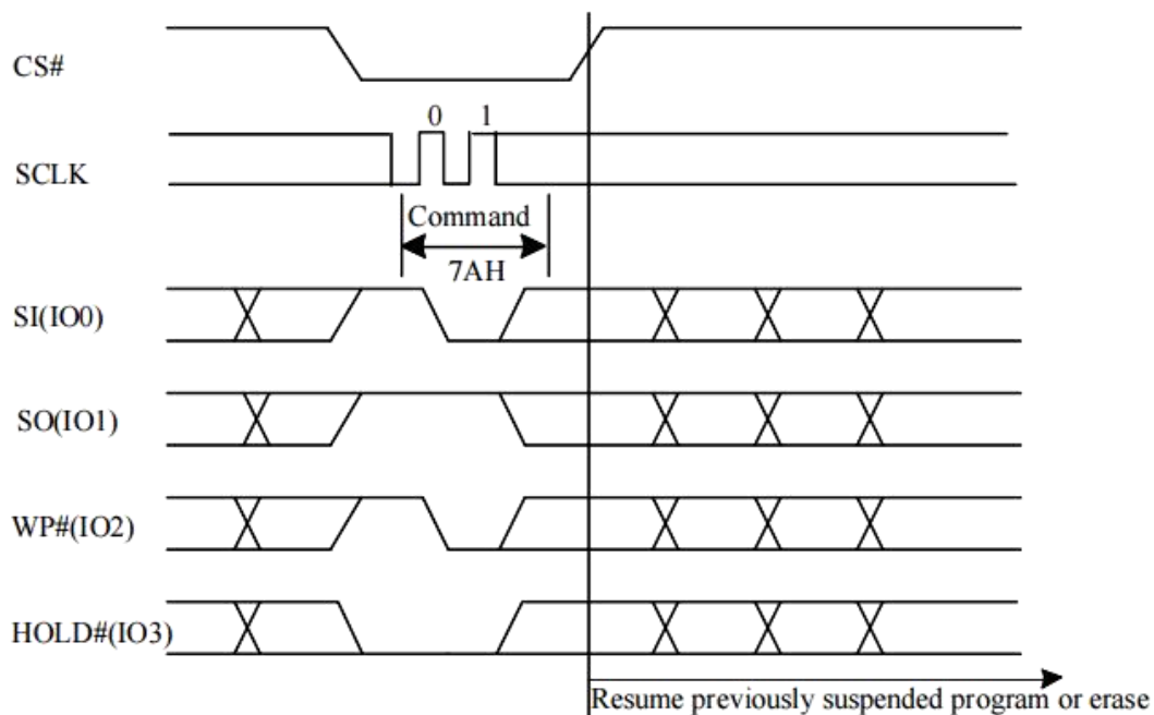
Figure 10-49a Resume to Read Latency (QPI)
