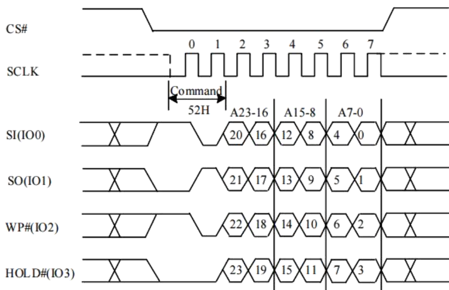
Figure 10-28a Block Erase 32K (BE32K) Sequence (QPI)
