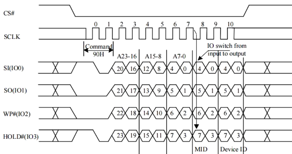
Figure 10-43a Read Electronic Manufacturer & Device ID (REMS) Sequence (QPI)
