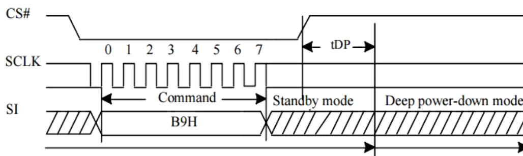
Figure 10-41 Deep Power-down (DP) Sequence (Command B9h)
