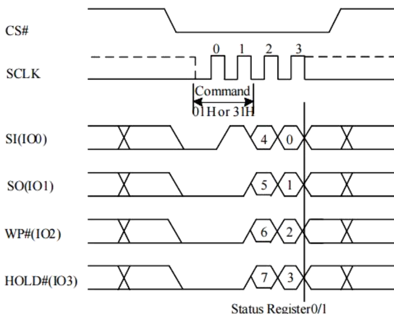
Figure 10-7a Write Status Register (WRSR) Sequence (QPI)
