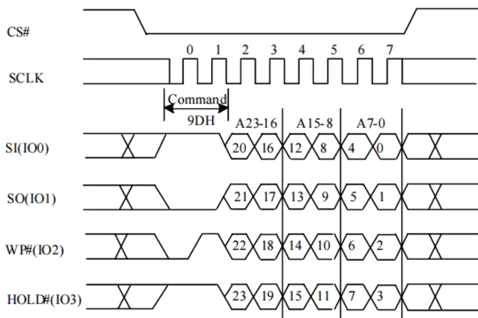
Figure 10-37a Buffer to Main Memory Page Program Sequence (QPI)
