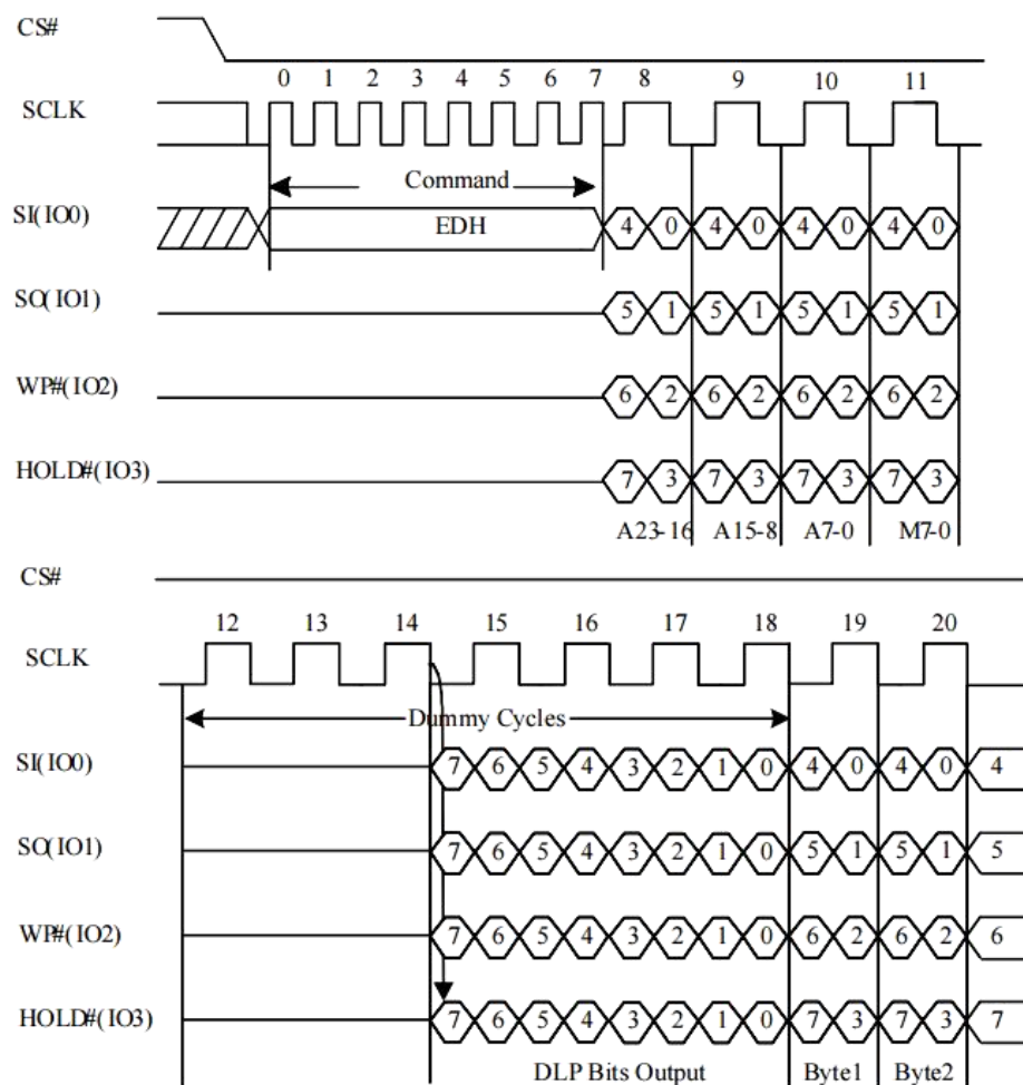
Figure 10-23g DTR 4IO Read with DLP bits output Sequence
