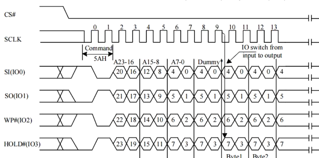
Figure 10-59a Read Serial Flash Discoverable Parameter (RDSFDP) Sequence (QPI)
