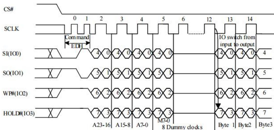
Figure 10-18b DTR 4IO Read Mode Sequence (QPI EDH M5-4 ≠ (1,0))
