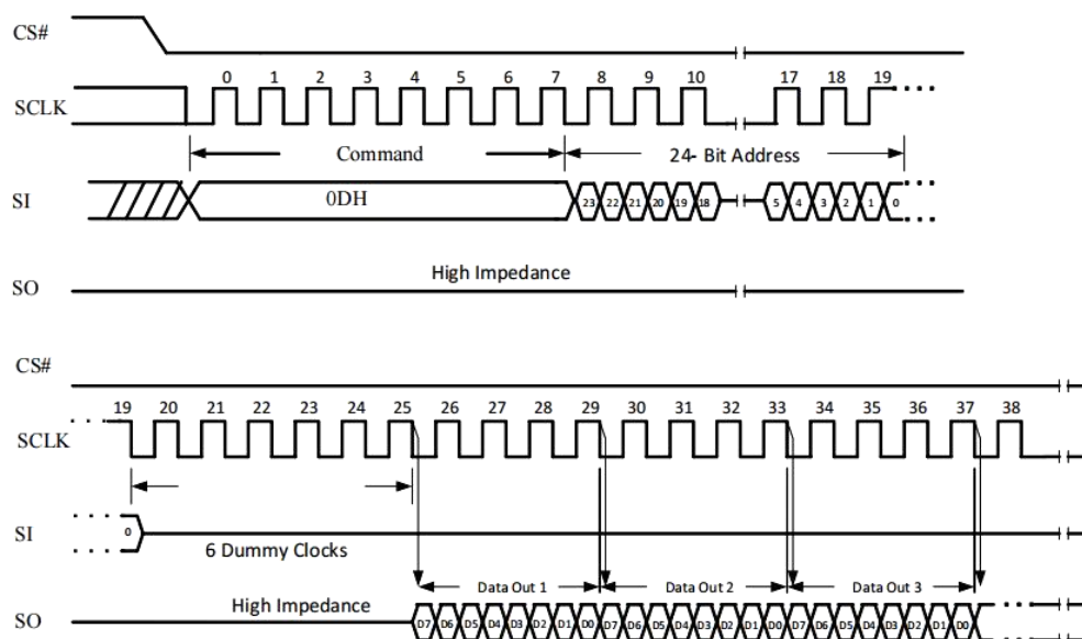
Figure 10-11 DTR Fast Read Sequence (Command 0Dh)
