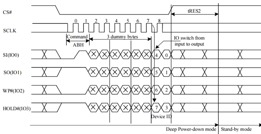
Figure 10-42a Read Electronic Signature (RES) Sequence (QPI)
