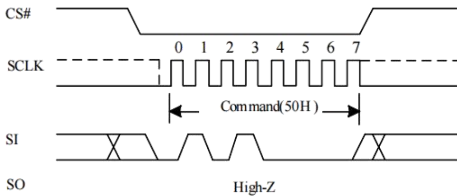
Figure 10-4 Write Enable for Volatile Status Register Sequence (Command 50h)
