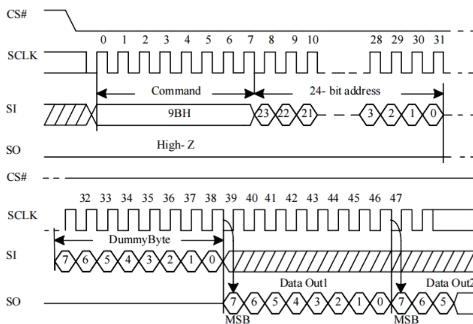
Figure 10-35 Buffer Read Sequence (Command 9Bh)
