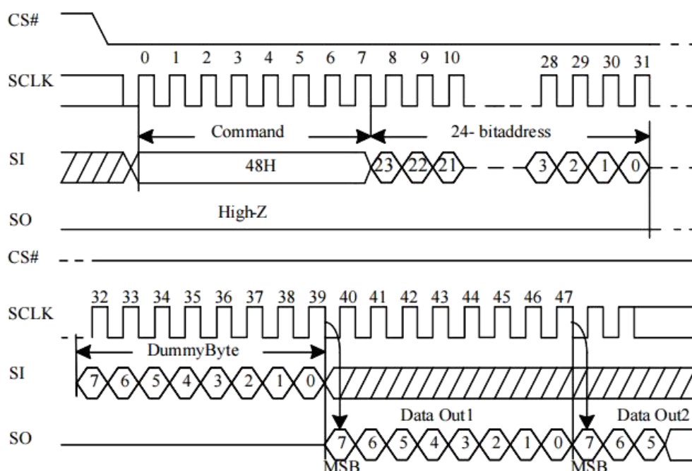
Figure 10-40 Read Security Registers(RDSCUR) Sequence (Command 48)
