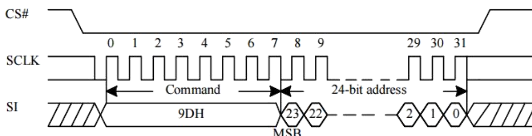
Figure 10-37 Buffer to Main Memory Page Program Sequence (Command 9Dh)
