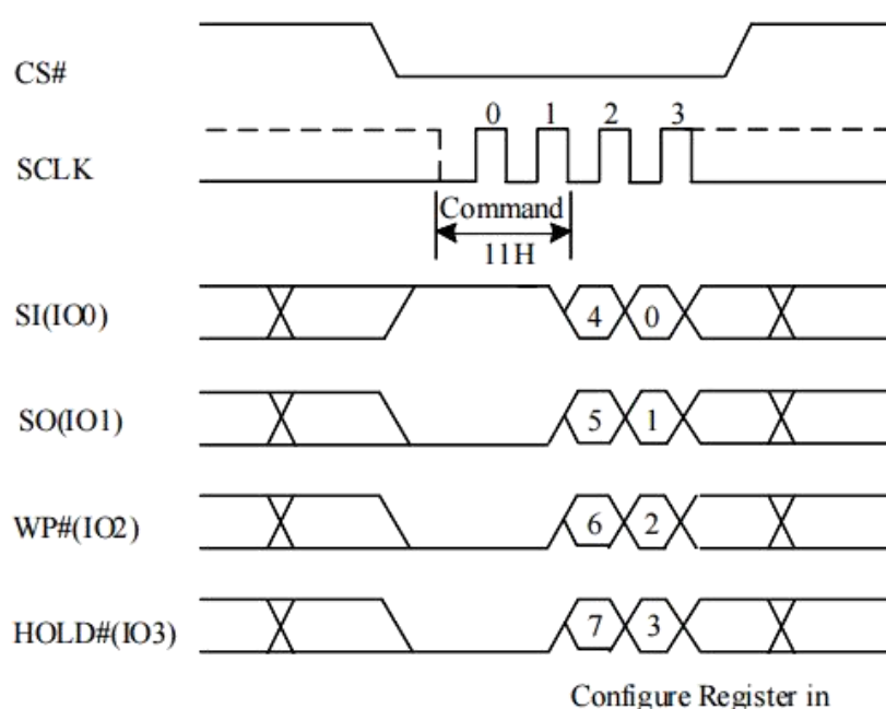
Figure 10-8a Write Configure Register (WRCR) Sequence (QPI)
