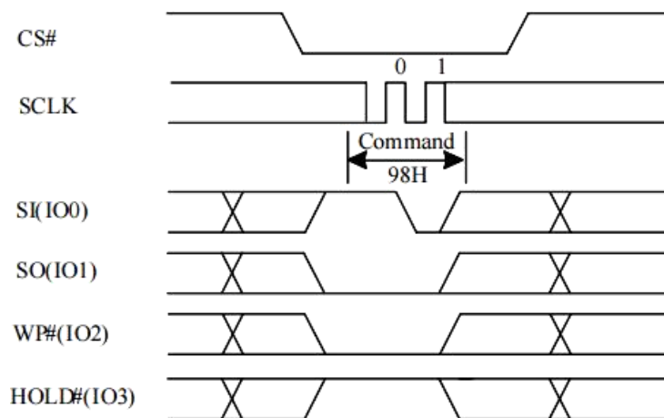
Figure 10-55a Global Block Unlock (QPI)
