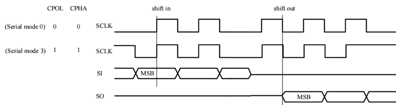
Figure 8-1 Serial Peripheral Interface Modes Supported
