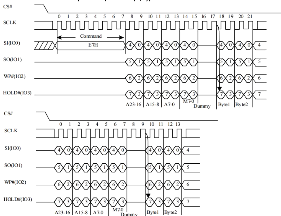
Figure 10-19a 4IO Word Read Sequence (M5-4 = (1,0))
