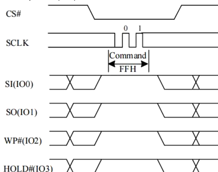
Figure 10-25a Disable QPI Sequence (QPI)
