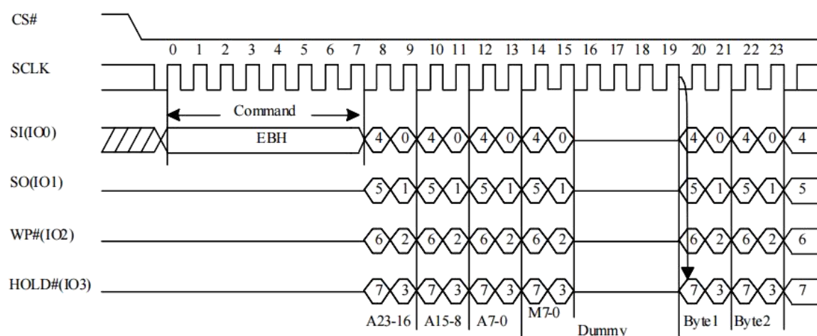
Figure 10-16 4IO Read Sequence (Command EBM5-4 ≠ (1,0))
