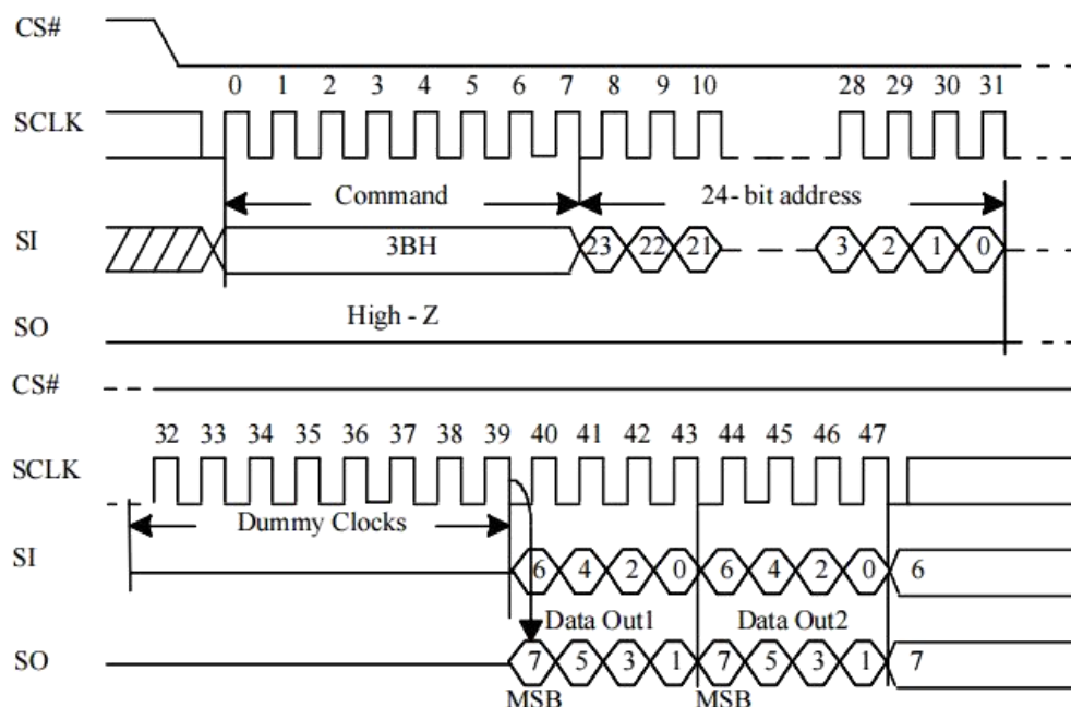
Figure 10-12 Dual Read Mode Sequence (Command 3Bh)
