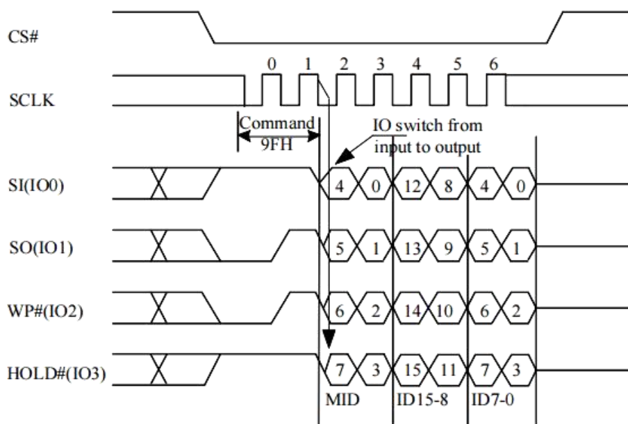
Figure 10-46a Read Identification (RDID) Sequence (QPI)
