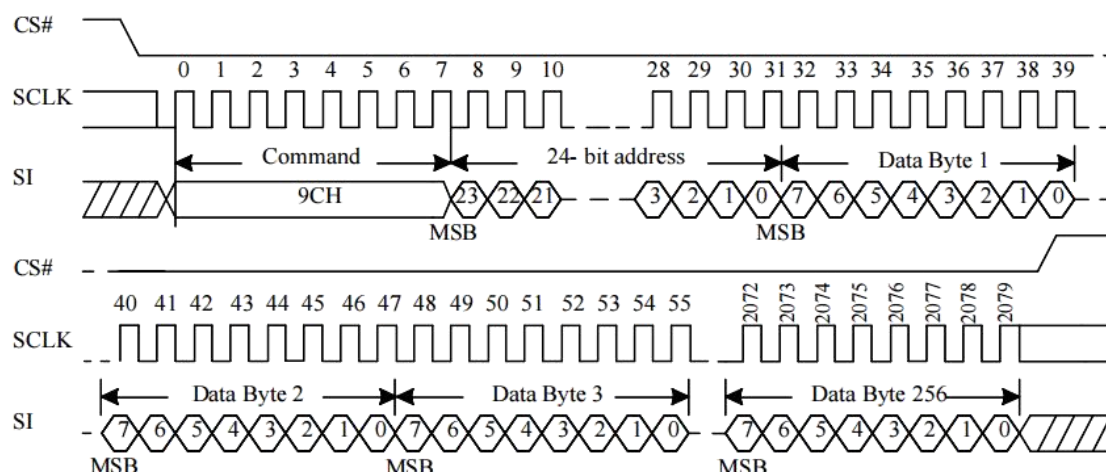
Figure 10-36 Buffer Write Sequence (Command 9Ch)
