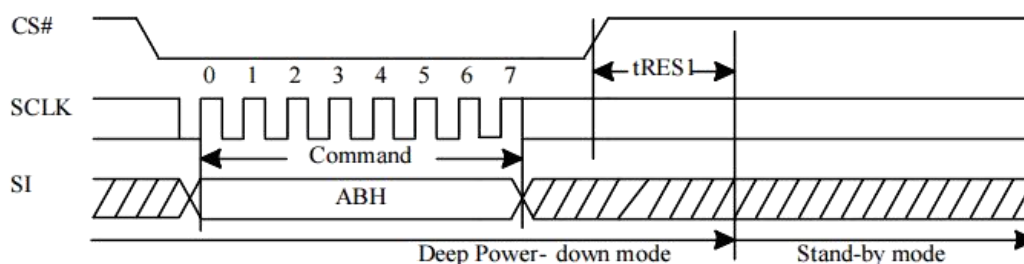
Figure 10-42b Release from Deep Power-down (RDP) Sequence (Command ABH)
