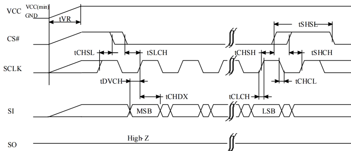
Figure 5-8 AC Timing at Device Power-Up
