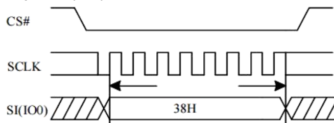
Figure 10-24 Enable QPI Sequence (38H)
