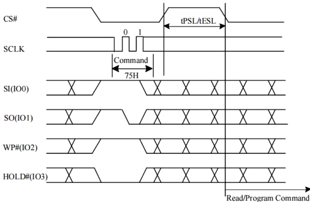
Figure 10-48a Suspend to Read/Program Latency (QPI)
