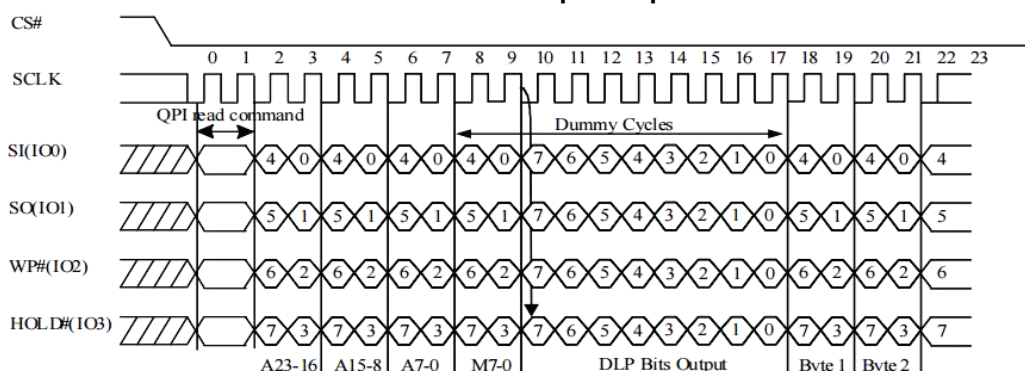
Figure 10-23d QPI Read instructions with DLP bits output Sequence
