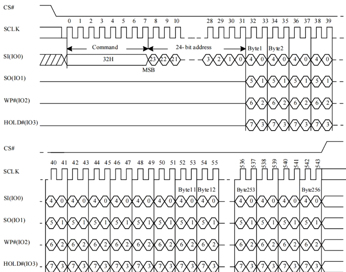
Figure 10-32 Quad Page Program (QPP) Sequence (Command 32h)
