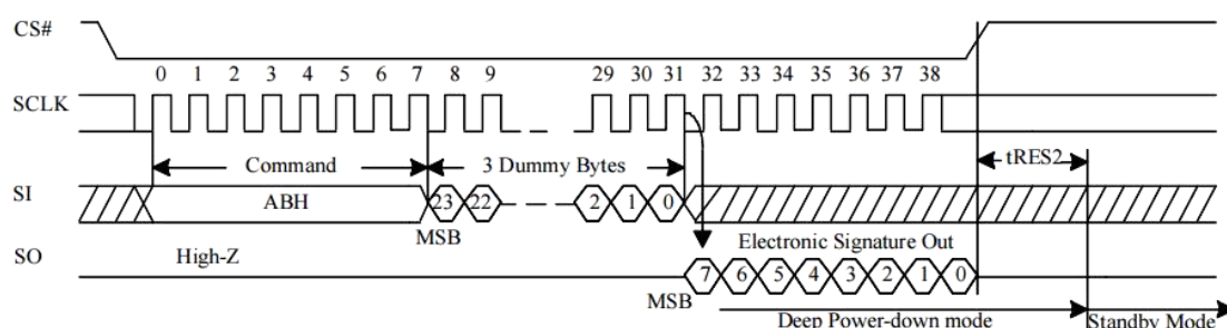
Figure 10-42 Read Electronic Signature (RES) Sequence (Command ABh)
