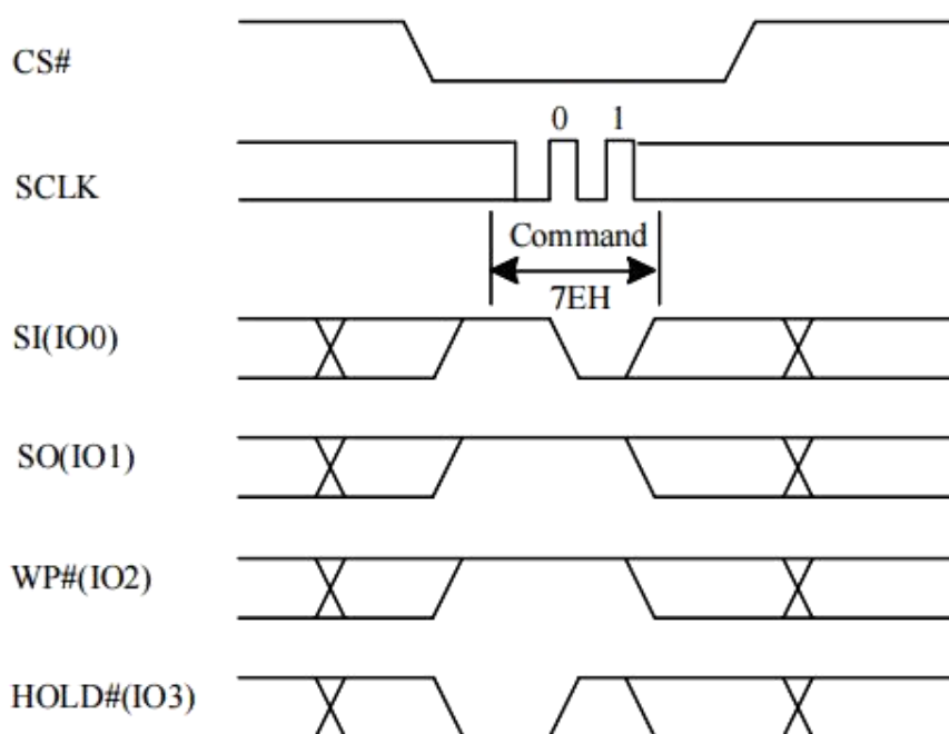
Figure 10-54a Global Block Lock (QPI)
