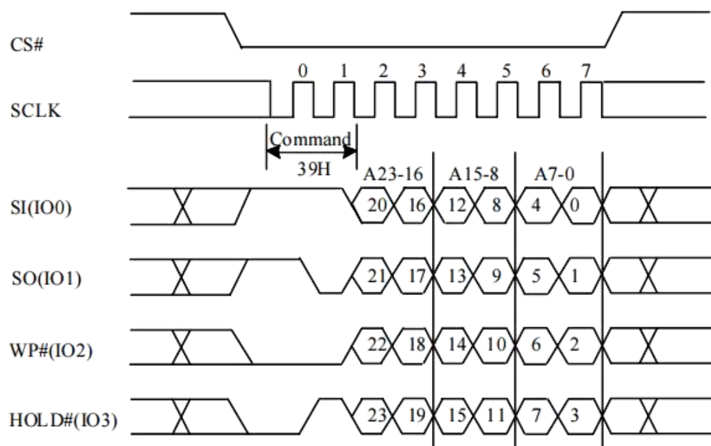
Figure 10-52a Individual Block Unlock (QPI)
