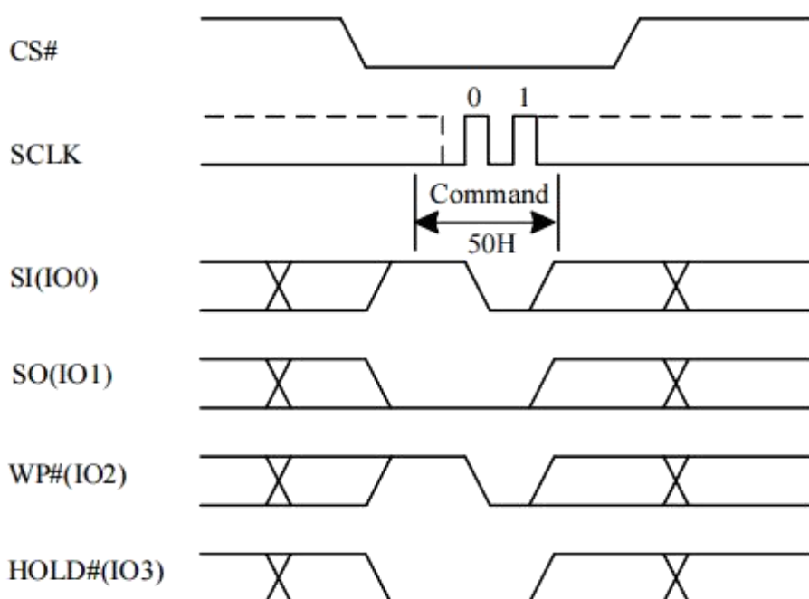
Figure 10-4a Write Enable for Volatile Status Register Sequence (QPI)
