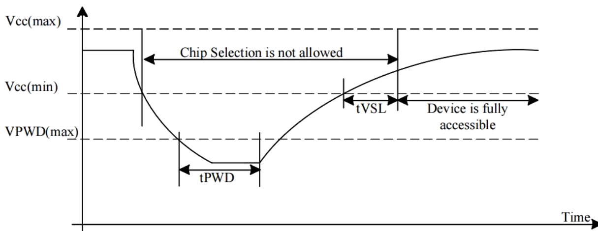
Figure 5-10 Power down-up Timing
