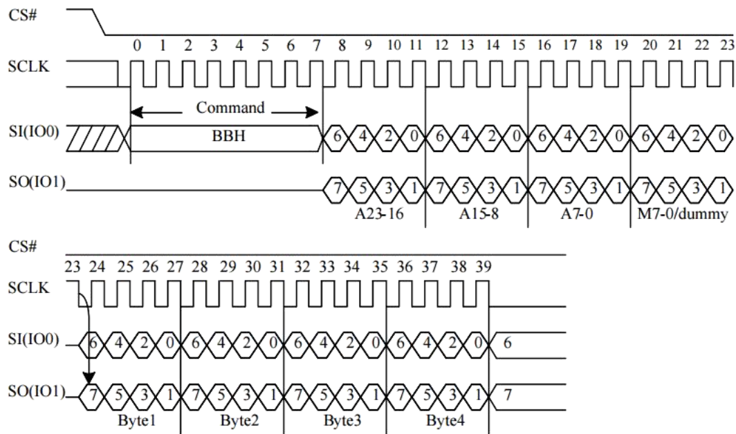
Figure 10-13 2IO Read Sequence (Command BBM5-4 ≠ (1,0))
