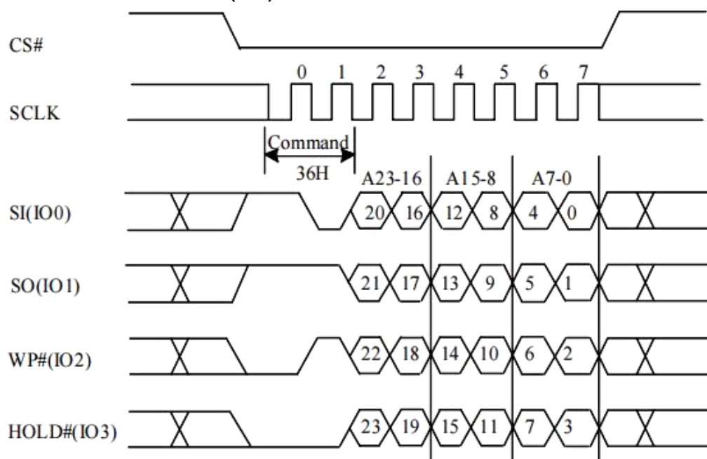
Figure 10-51a Individual Block Lock (QPI)
