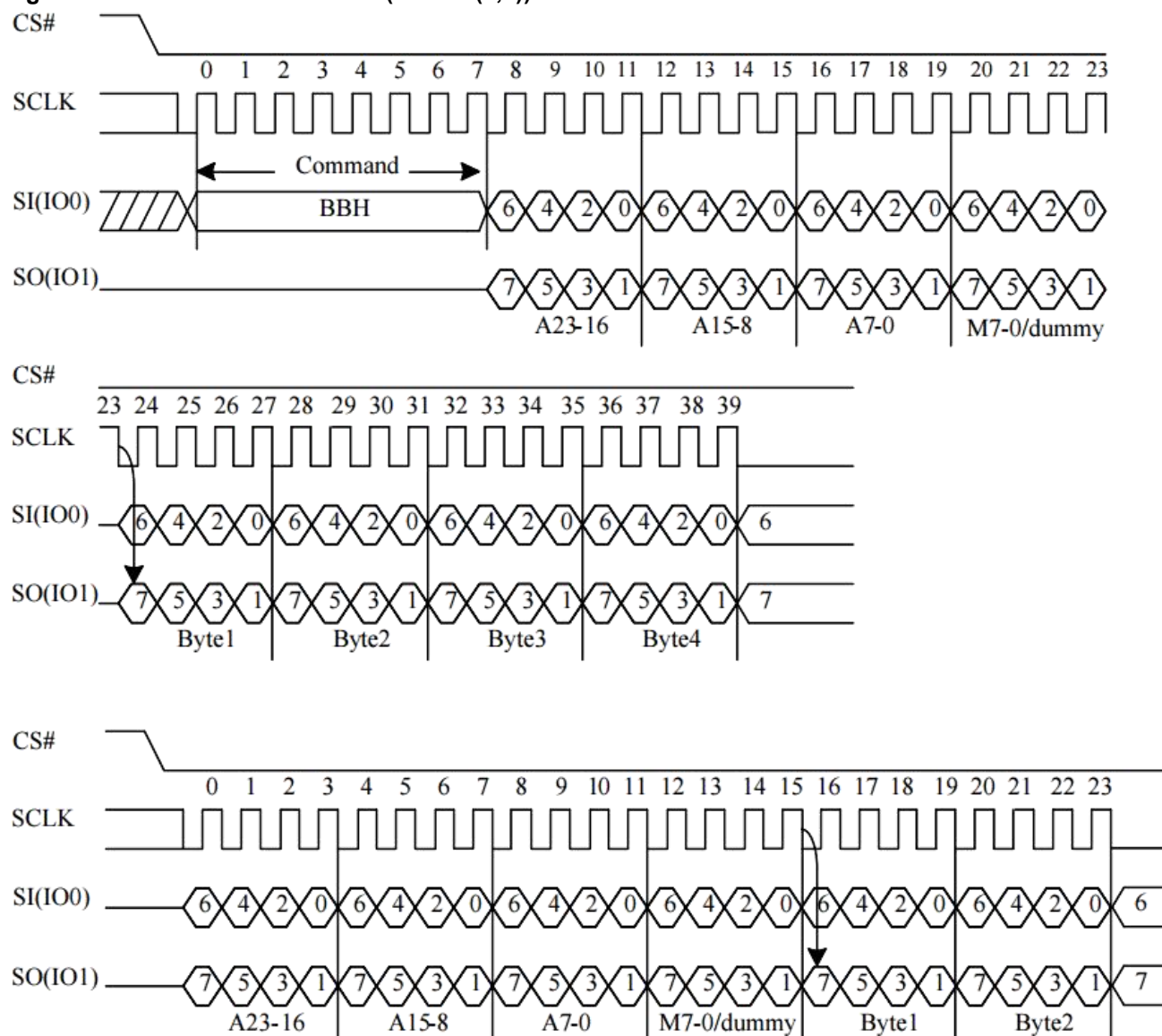
Figure 10-13a 2IO Continue Read (M5-4 = (1,0))
