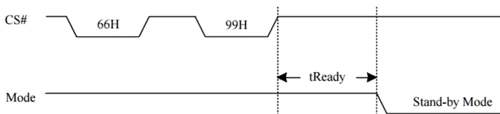
Figure 10-56a Reset Sequence
