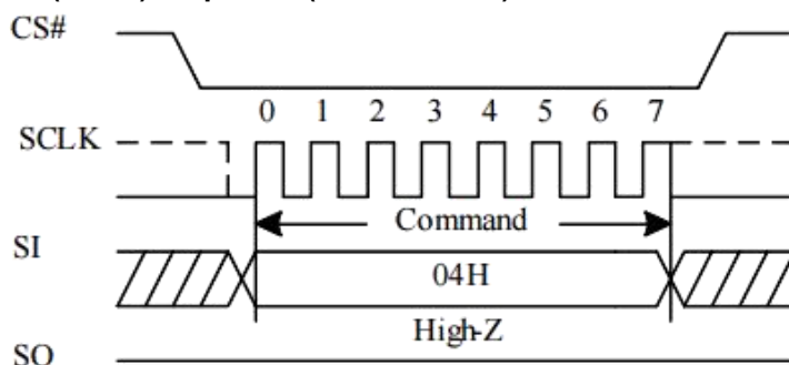
Figure 10-3 Write Disable (WRDI) Sequence (Command 04)
