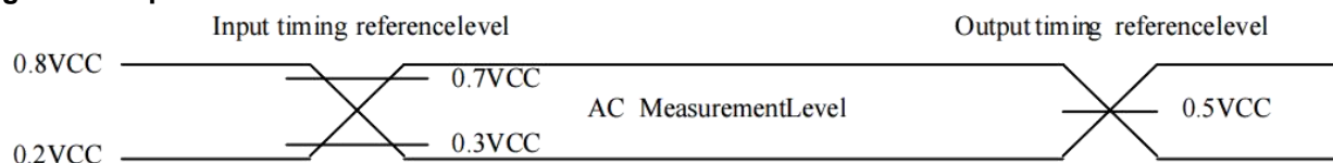
Figure 5-1 Input Test Waveforms and Measurement Level
