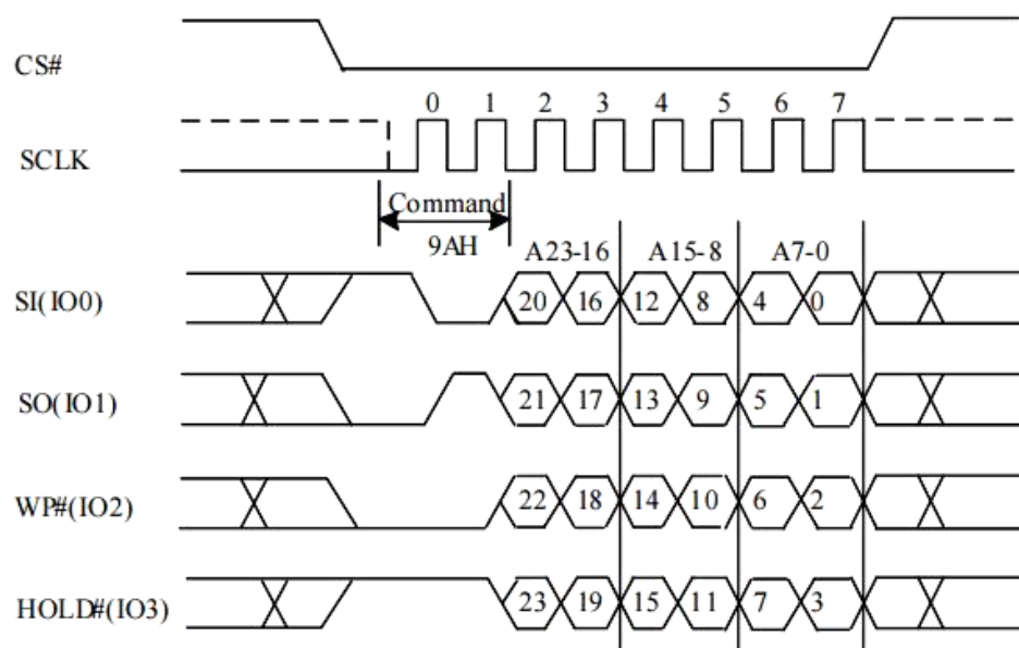
Figure 10-35a Buffer Load Sequence (QPI)
