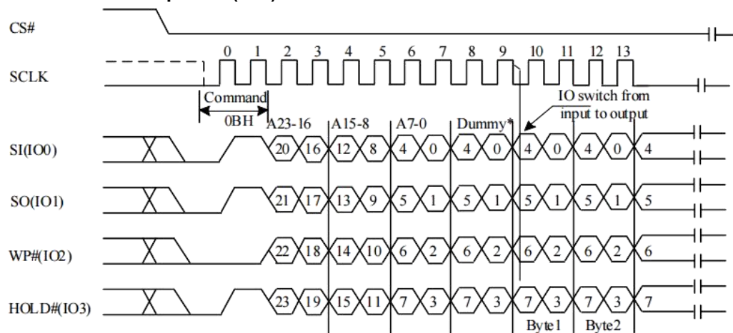
Figure 10-10a Fast Read Sequence (QPI)
