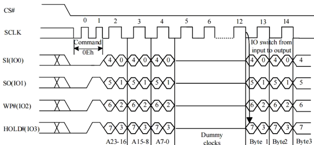
Figure 10-22 Burst Read with Wrap Sequence (QPI)
