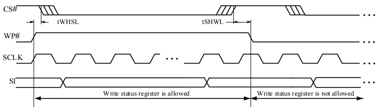
Figure 5-7 WP Timing
