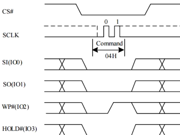
Figure 10-3a Write Disable (WRDI) Sequence (QPI)
