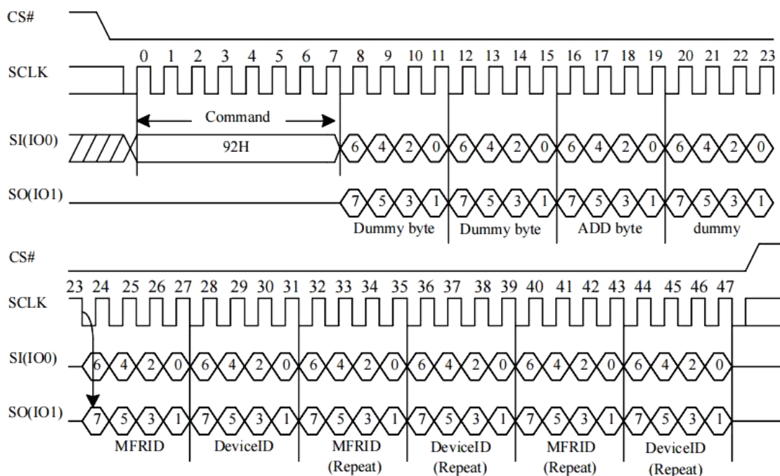
Figure 10-44 DUAL I/O Read Electronic Manufacturer & Device ID (DREMS) Sequence (Command 92h)
