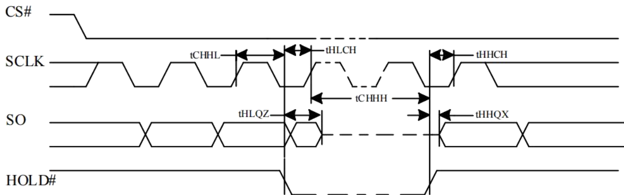
Figure 5-6 Hold Timing
