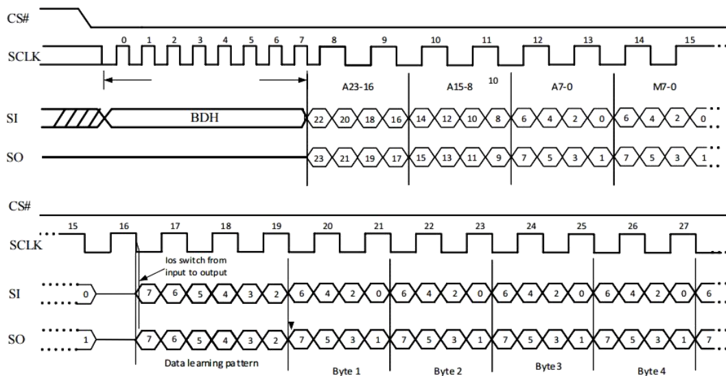
Figure 10-23f DTR 2IO Read with DLP bits output Sequence
