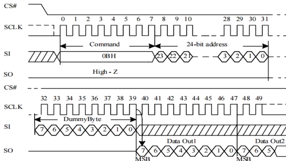
Figure 10-10 Fast Read (FREAD) Sequence (Command 0Bh)
