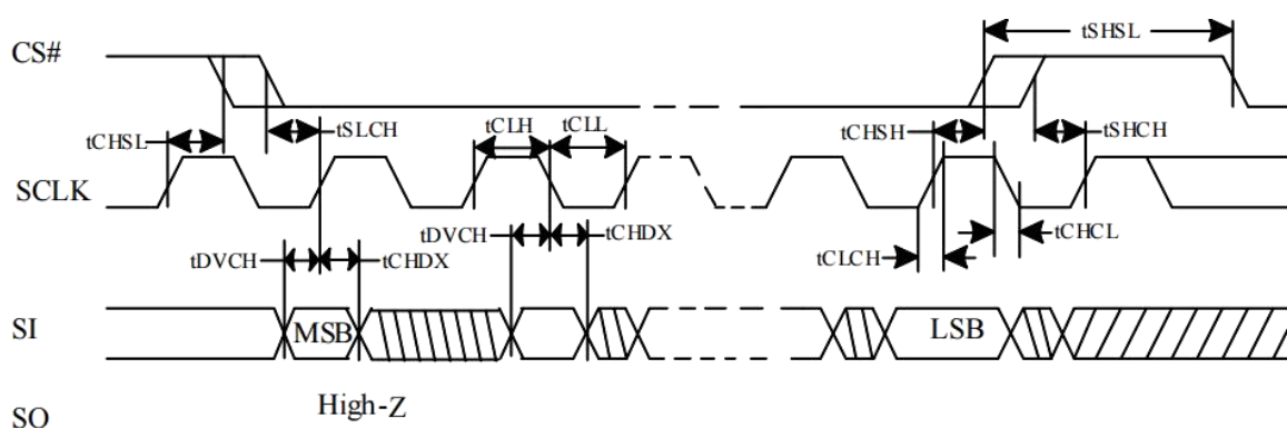
Figure 5-4b Serial Input Timing in DTR Mode
