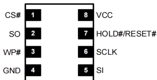
DFN-8 4*4/DFN-8 5*6
