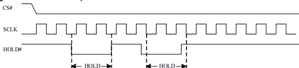
Figure 9-1 Hold Condition Operation
