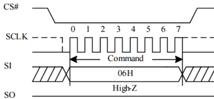
Figure 10-2 Write Enable (WREN) Sequence (Command 06)
