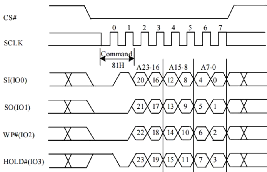
Figure 10-26a Page Erase Sequence (QPI)
