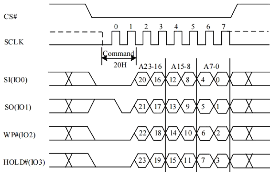
Figure 10-27c Sector Erase (SE) Sequence (QPI)
