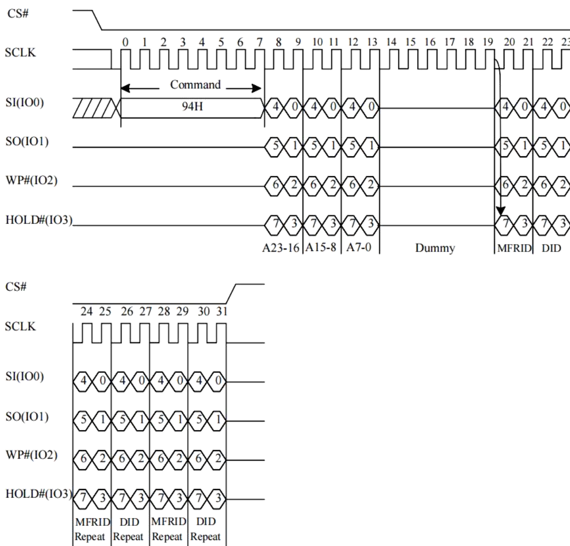
Figure 10-45 QUAD I/O Read Electronic Manufacturer & Device ID (QREMS) Sequence (Command 94h)
