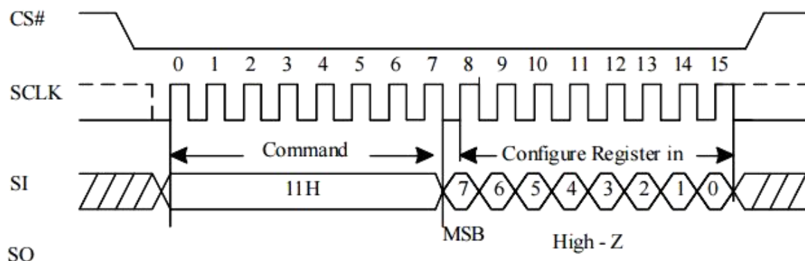
Figure 10-8 Write Configure Register (WRCR) Sequence (Command 11h)
