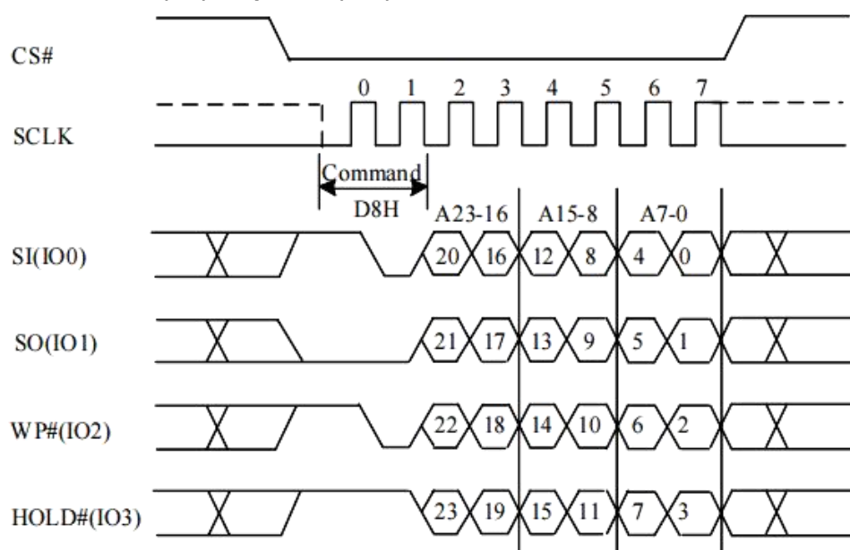
Figure 10-29a Block Erase (BE) Sequence (QPI)
