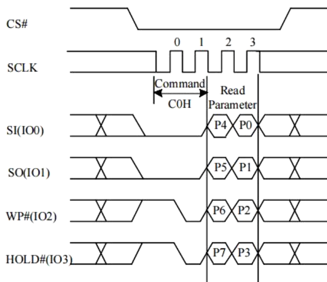
Figure 10-20 Set Read Parameters Sequence (QPI)
