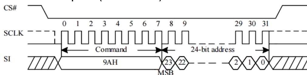
Figure 10-34 Buffer Load Sequence (Command 9Ah)
