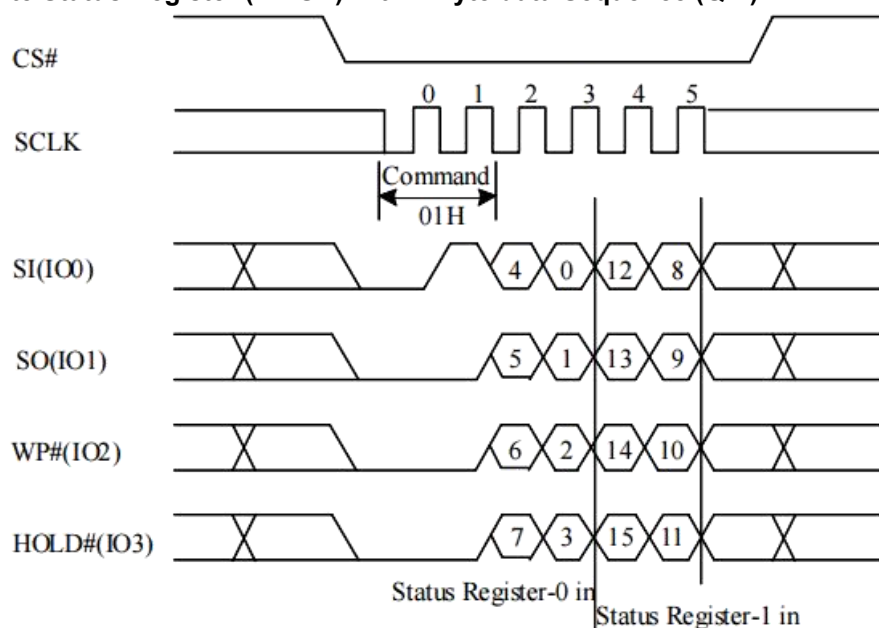
Figure 10-7b Write Status Register (WRSR) with 2 Byte data Sequence (QPI)
