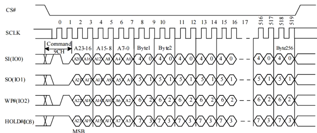
Figure 10-36a Buffer Write Sequence (QPI)
