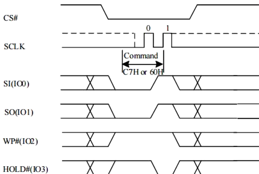
Figure 10-30a Chip Erase (CE) Sequence (QPI)
