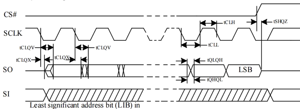
Figure 5-5 Output Timing
