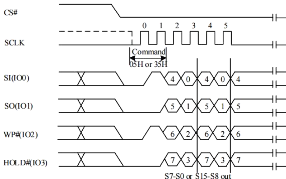
Figure 10-5a Read Status Register (RDSR) Sequence (QPI)
