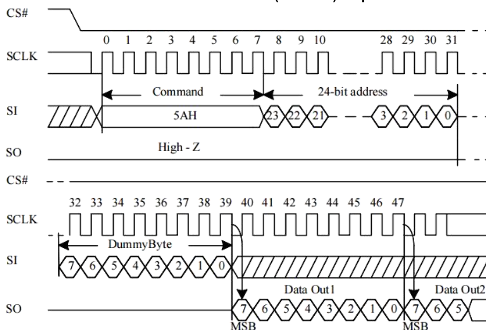
Figure 10-59 Read Serial Flash Discoverable Parameter (RDSFDP) Sequence
