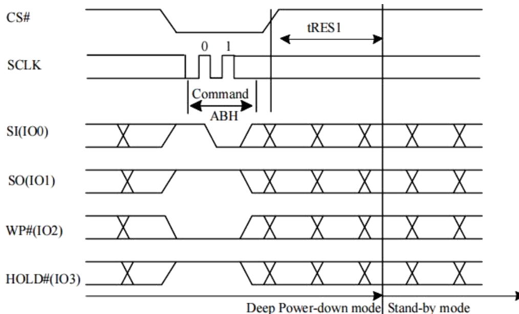
Figure 10-42c Release from Deep Power-down (RDP) Sequence (QPI)
