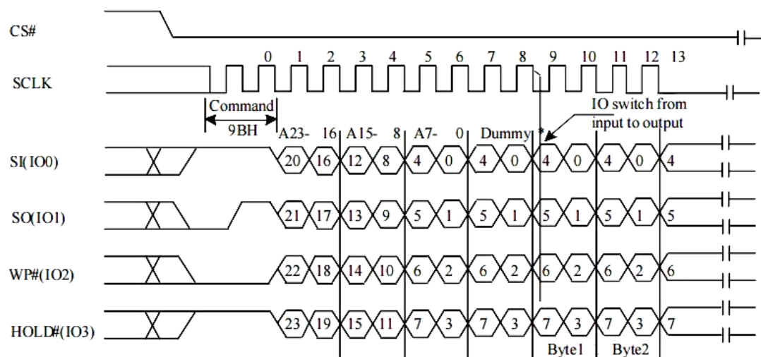
Figure 10-35a Buffer Read Sequence (QPI)
