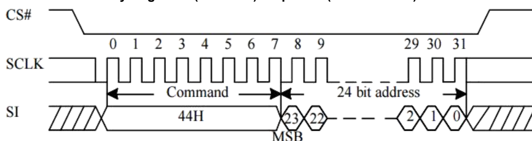
Figure 10-38 Erase Security Registers (ERSCUR) Sequence (Command 44)
