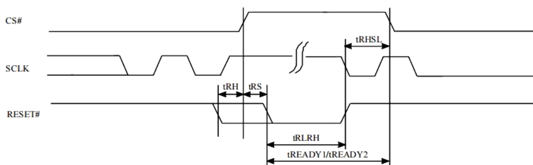
Figure 10-57 RESET Timing
