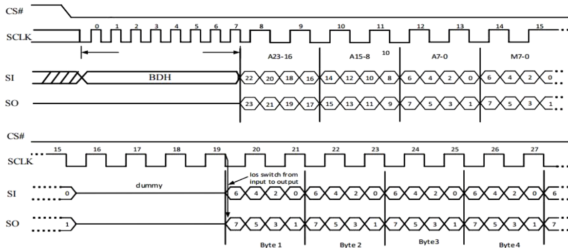
Figure 10-14 DTR 2IO Read Sequence (Command BDM5-4 ≠ (1,0))
