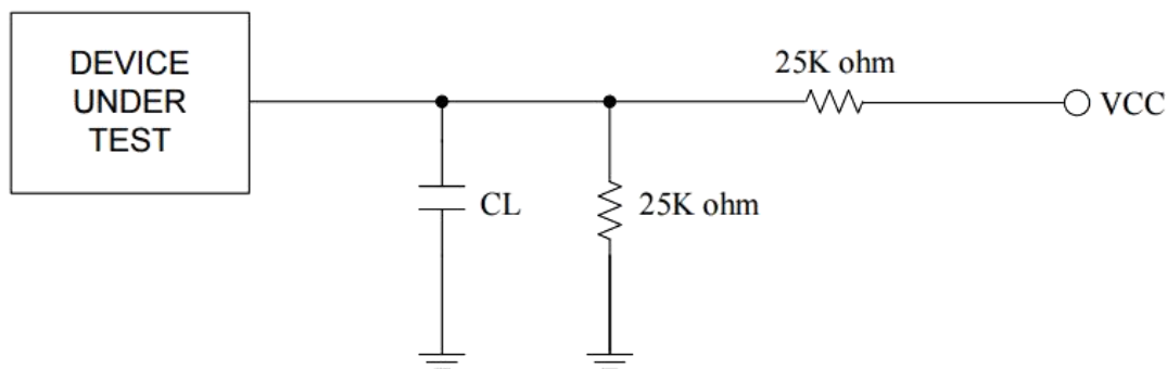
Figure 5-2 Output Loading
