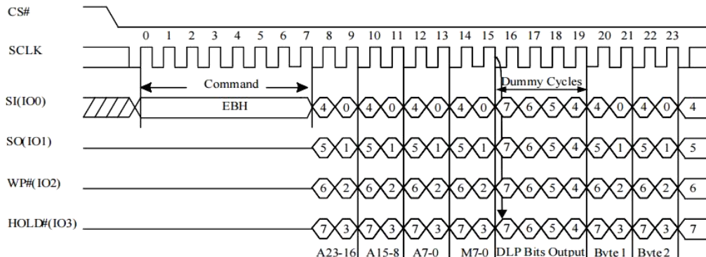
Figure 10-23c 4IO Read with DLP bits output Sequence
