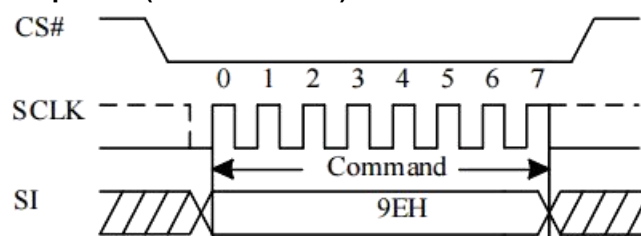
Figure 10-33 Buffer Clear Sequence (Command 9EH)
