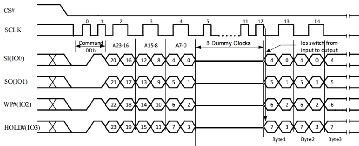
Figure 10-11a DTR Fast Read Sequence (QPI)
