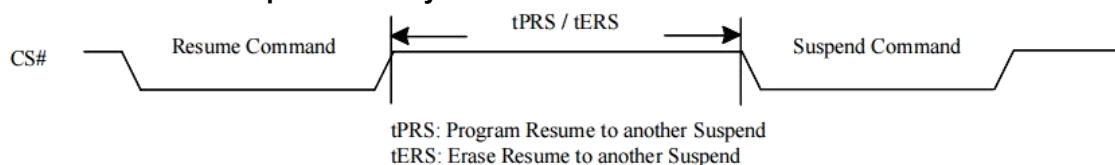
Figure 10-47 Resume to Suspend Latency
