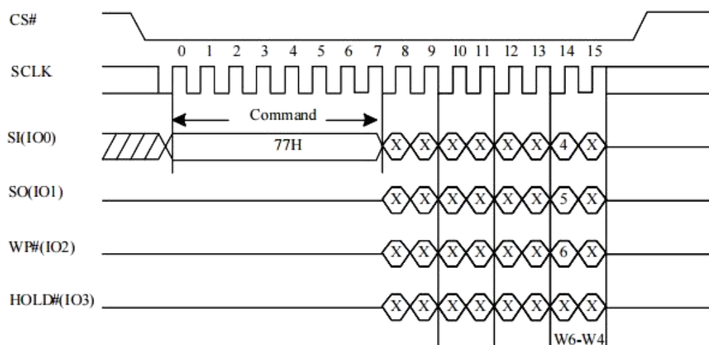
Figure 10-17 Set Burst Read (SBL) Sequence (Command 77h)
