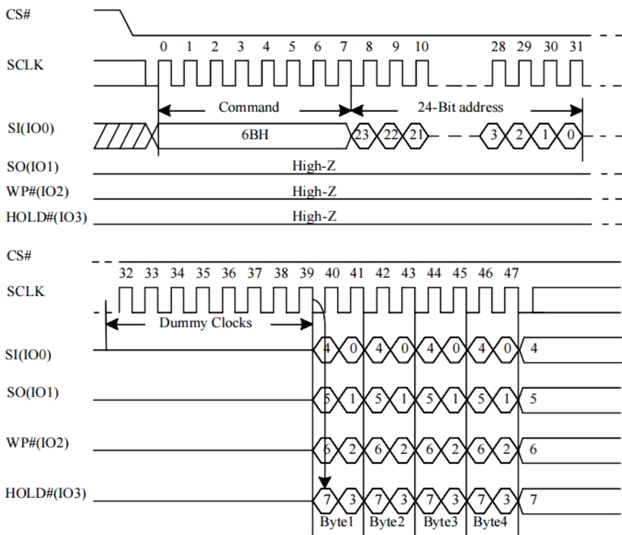
Figure 10-15 Quad Read Sequence (Command 6Bh)
