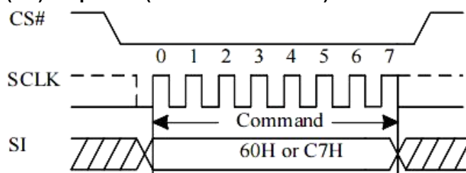
Figure 10-30 Chip Erase (CE) Sequence (Command 60 or C7)
