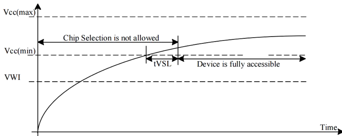
Figure 5-9 Power-up Timing
