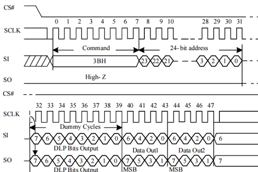
Figure 10-23a Dual Read with DLP bits output Sequence
