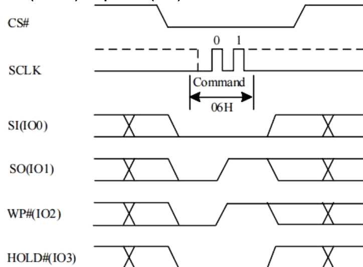
Figure 10-2a Write Enable (WREN) Sequence (QPI)
