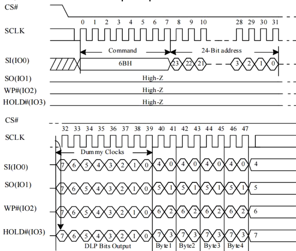
Figure 10-23b Quad Read with DLP bits output Sequence
