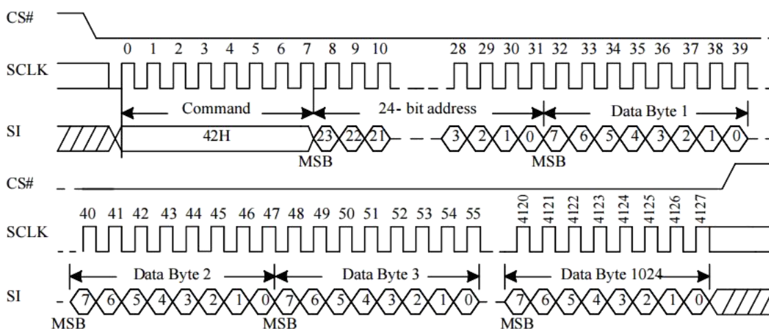
Figure 10-39 Program Security Registers (PRSCUR) Sequence (Command 42h)
