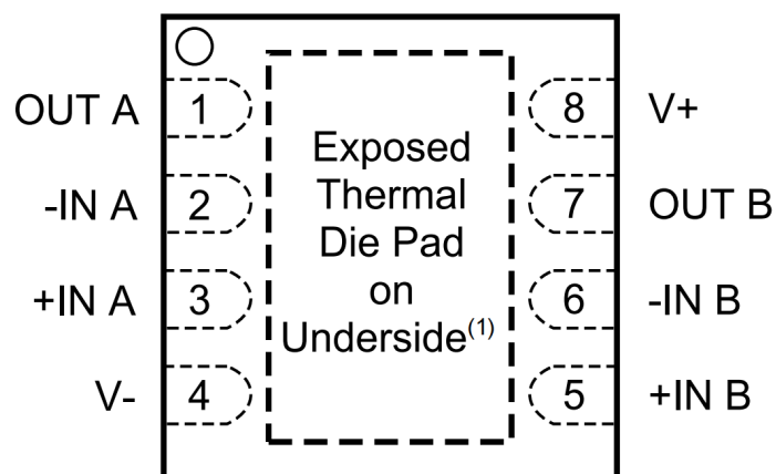
QFN-8(2*2) Pin Diagram
