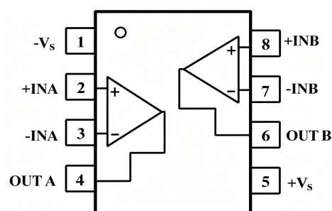
TSV912 SOT23-8 Pin Diagram
