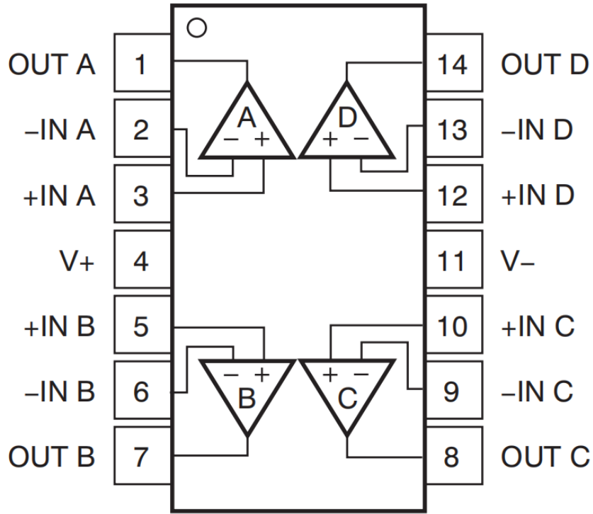
TSV914 SOP14/TSSOP14 Pin Diagram
