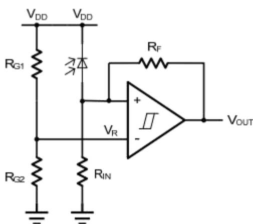
Figure 6. IR Receiver
