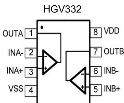
SOP-8/MSOP-8
