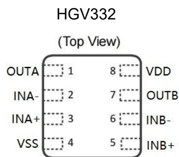
DFN-8 3*3
