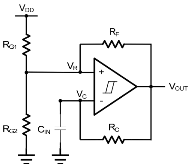
Figure 7. Oscillator
