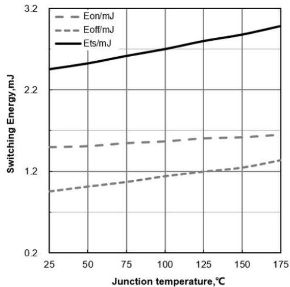
Figure 12. Typical Switching Energy vs Junction Temperature ( V_{CE}=400\text{V} , V_{GE}=15/0\text{V} , I_C=80\text{A} )
