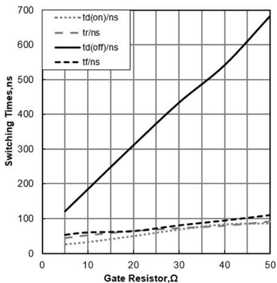
Figure 9. Typical Switching Times vs Gate Resistor ( T_J=25^{\circ}\text{C} , V_{CE}=400\text{V} , V_{GE}=15/0\text{V} , I_C=80\text{A} )
