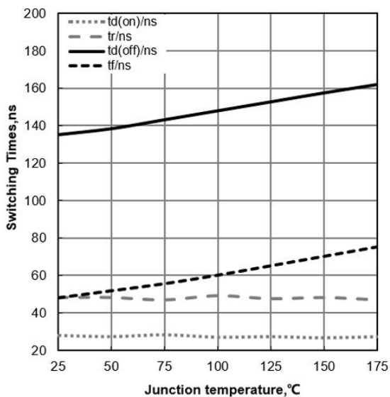
Figure 11. Typical Switching Times vs Junction Temperature ( V_{CE}=400\text{V} , V_{GE}=15/0\text{V} , I_C=80\text{A} )
