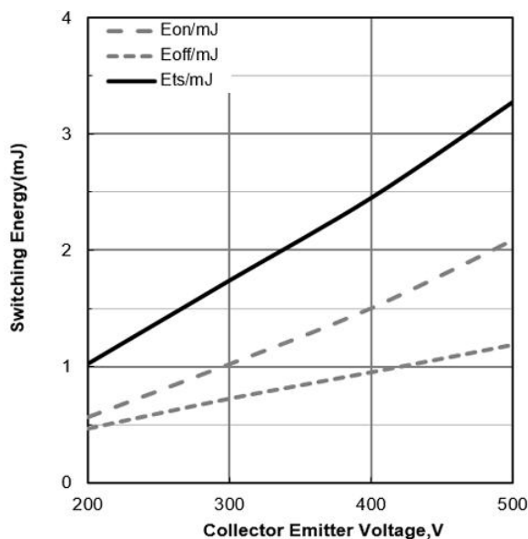
Figure 16. Typical Switching Energy vs VCE ( T_J=25^\circ\text{C} , V_{GE}=15/0\text{V} , I_C=80\text{A} )
