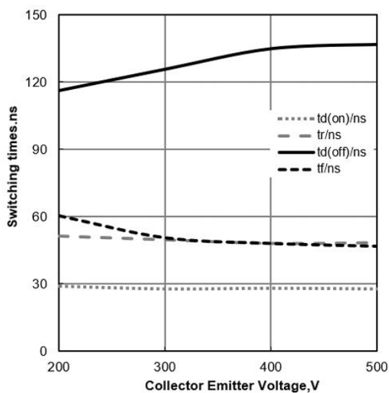
Figure 15. Typical Switching Times vs VCE ( T_J=25^\circ\text{C} , V_{GE}=15/0\text{V} , I_C=80\text{A} )
