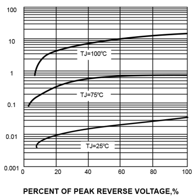
FIG. 4-TYPICAL REVERSE CHARACTERISTICS
