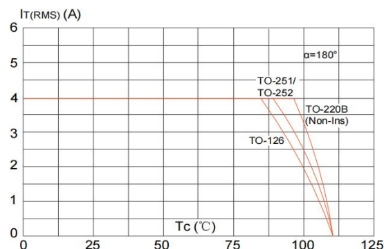
RMS on-state current versus case temperature
