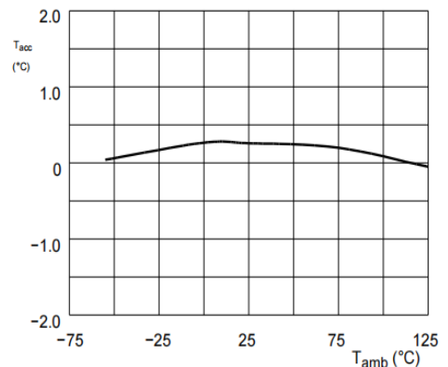
Figure 15. Typical temperature measurement accuracy with VCC = 3.3 V
