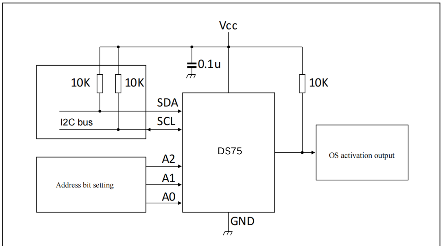
Figure 8. Typical Application
