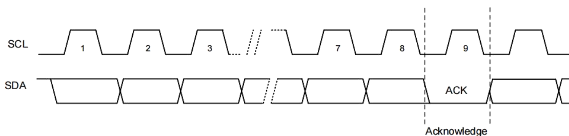
Figure 4-3 Output Acknowledge
