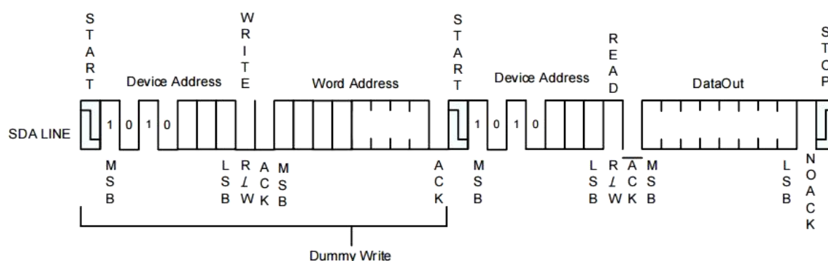
Figure 5-4 Random Read
