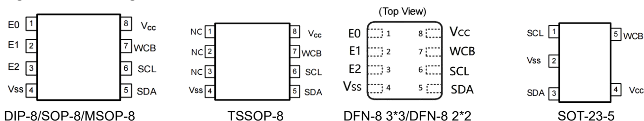
Figure 1-1 Pin Configuration
