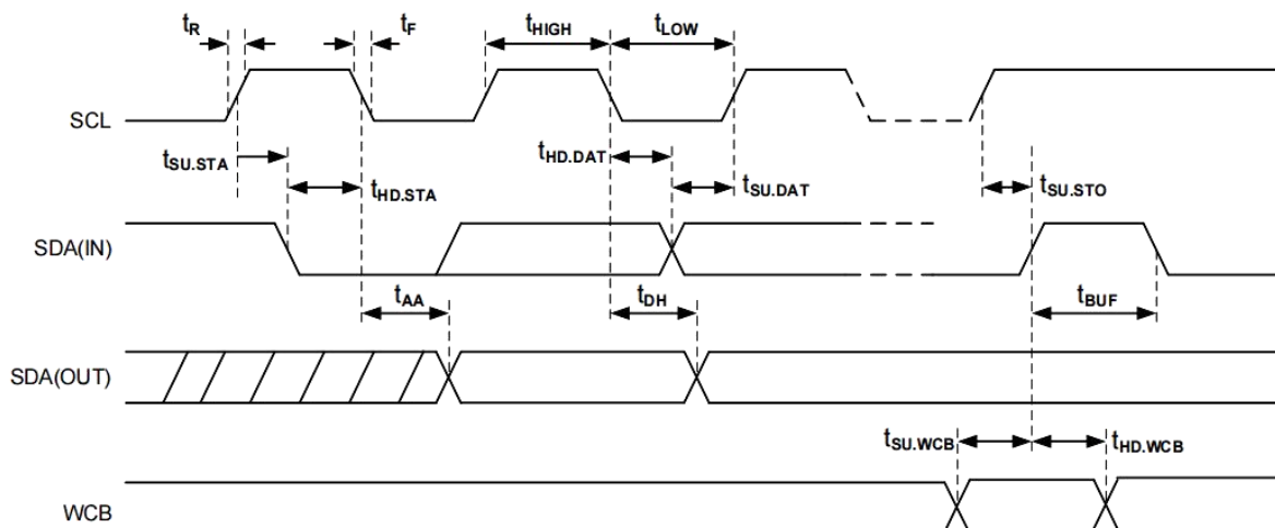
Figure 3-1 Bus Timing
