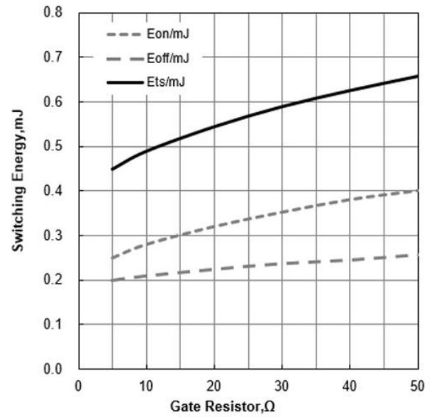
Figure 10. Typical Switching Energy vs Gate Resistor ( T_J=25^{\circ}\text{C} , V_{CE}=400\text{V} , V_{GE}=15/0\text{V} , I_C=10\text{A} )
