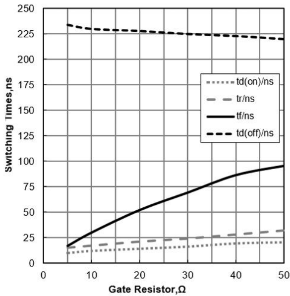
Figure 9. Typical Switching Times vs Gate Resistor ( T_J=25^{\circ}\text{C} , V_{CE}=400\text{V} , V_{GE}=15/0\text{V} , I_C=10\text{A} )
