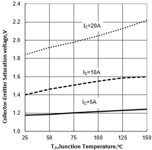
Figure 7. Typical Collector-Emitter Saturation Voltage vs Junction Temperature ( V_{GE}=15\text{V} )
