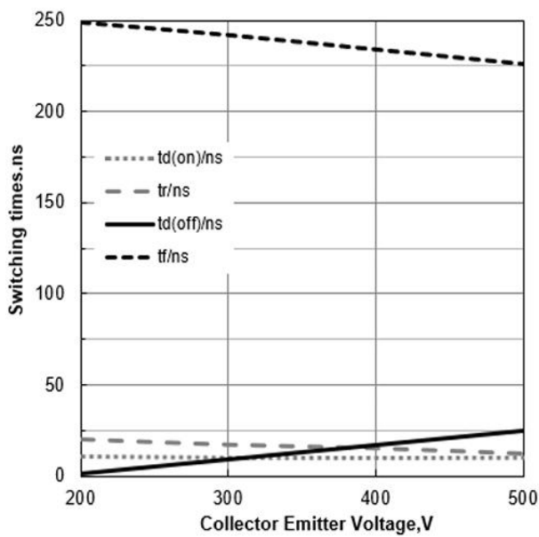
Figure 15. Typical Switching Times vs V_{CE} ( T_J=25^\circ\text{C} , V_{GE}=15/0\text{V} , I_C=10\text{A} )
