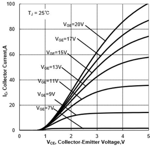
Figure 5. Typical Output Characteristics ( T_J=25^\circ\text{C} )
