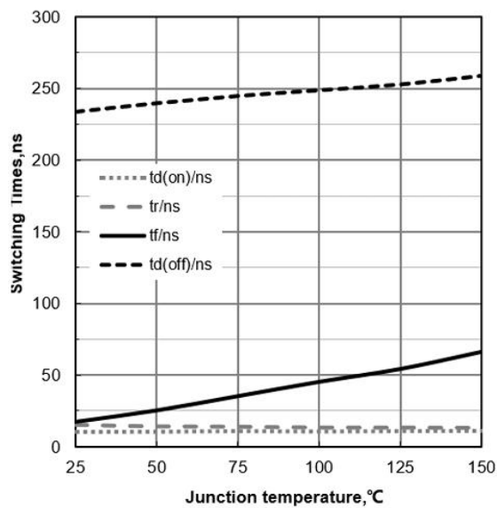
Figure 11. Typical Switching Times vs Junction Temperature ( V_{CE}=400\text{V} , V_{GE}=15/0\text{V} , I_C=10\text{A} )
