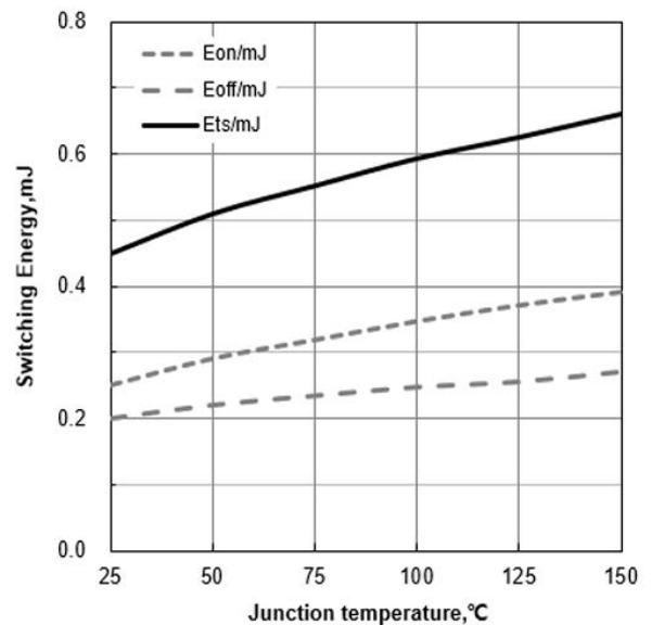
Figure 12. Typical Switching Energy vs Junction Temperature ( V_{CE}=400\text{V} , V_{GE}=15/0\text{V} , I_C=10\text{A} )
