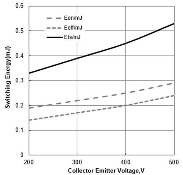
Figure 16. Typical Switching Energy vs V_{CE} ( T_J=25^\circ\text{C} , V_{GE}=15/0\text{V} , I_C=10\text{A} )
