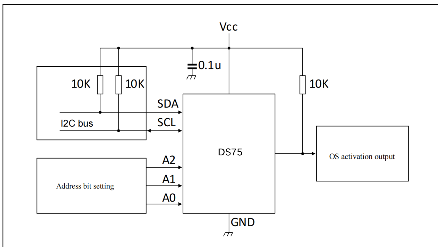
Figure 8. Typical Application
