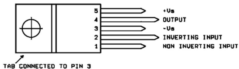
TO-220B-5
