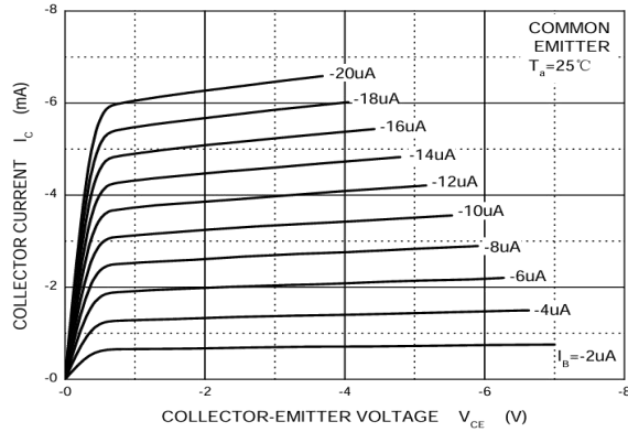
Static Characteristic
