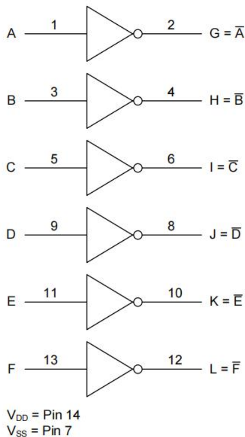
Figure 3.1: CD4069 Logic Diagram
