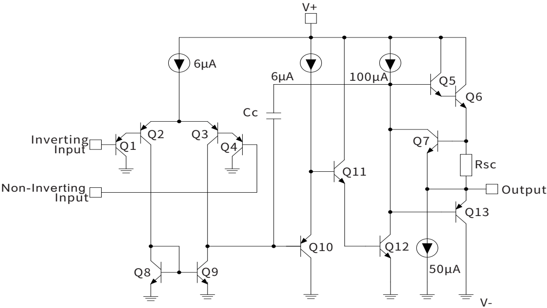
Figure 1.Internal Block Diagram
