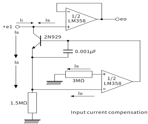
Fig.8 Using Symmetrical Amplifiers to Reduce Input Current
