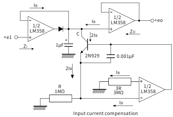
Fig.9 Low Drift Peak Detector
