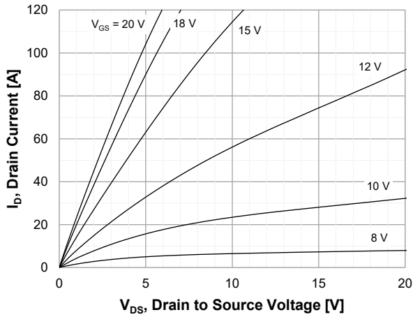
Figure 3. On-Region Characteristics T_J = 125^{\circ}\text{C}
