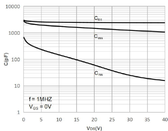
Figure 6: Capacitance Characteristics
