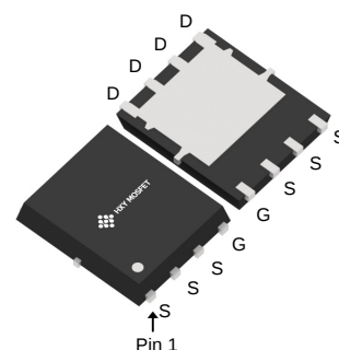
DFN5X6-8L (TDSON-8)
