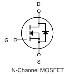
DFN5X6-8L (PQFN-8(4.9x5.8))
