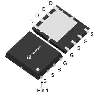
DFN5X6-8L (WPAK-8)
