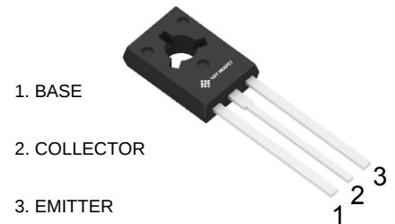
TO-126
