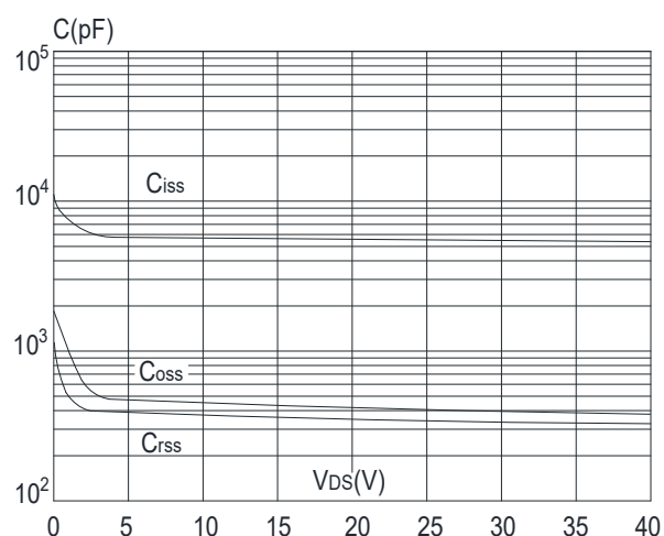
Figure 6: Capacitance Characteristics
