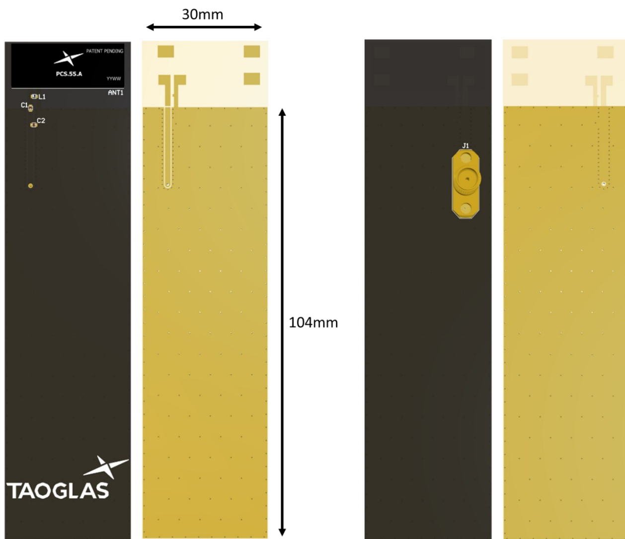
Top Side (PCS.55.A placement on 104x30mm PCB reference design)
