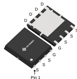
DFN5X6-8L (Power(5x6))
