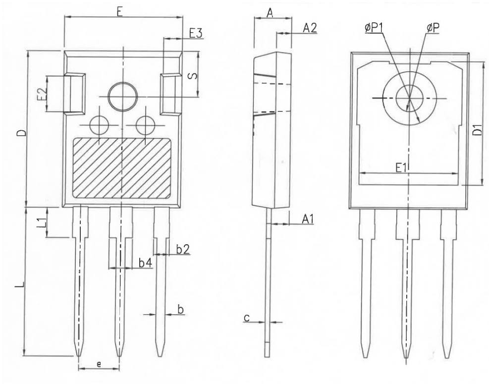
COMMON DIMENSIONS
