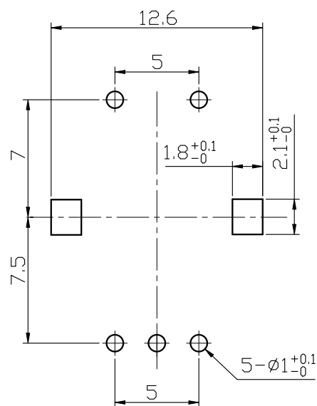
P. C. B. MOUNTING DETAIL
