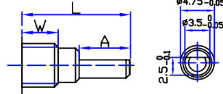
FK Shaft Style
