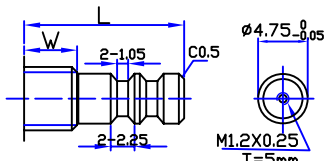
SM Shaft Style
