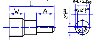
FT Shaft Style
