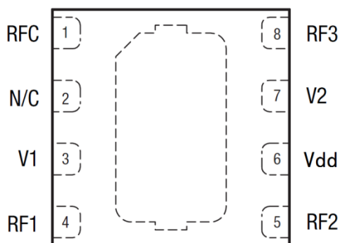
Figure 1. GSR1330S Pin-Def. (Top View)
