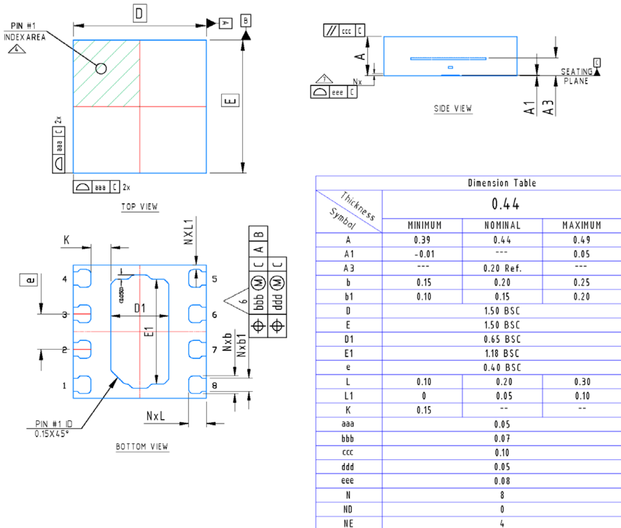
Figure 3. GSR1330S Package Dimensions
