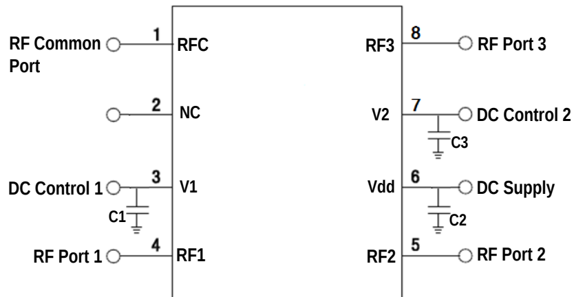
Figure 2. GSR1330S Evaluation Board Schematic
